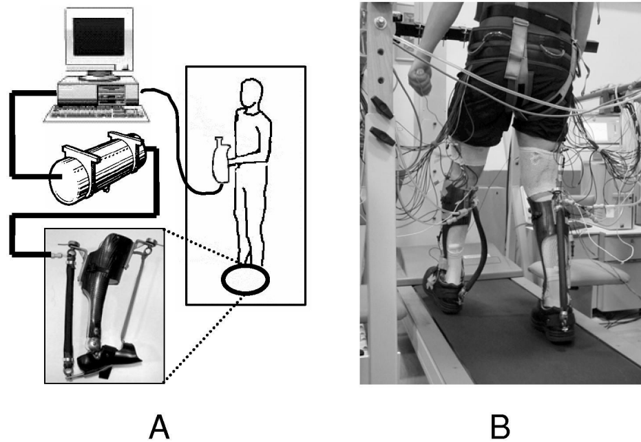
Figure 6. Pneumatically powered orthoses at the University of Michigan. A. The patient controls the timing of assistance with push buttons in each hand through an algorithm programmed on a remote computer. The computer commands airflow into and out of the pneumatic actuators attached to the orthoses, producing assistive torque at the ankle joint. B. A patient uses the push button controllers to assist walking on a treadmill. Source: Original figure from the Human Neuromechanics Laboratory at the University of Michigan.
