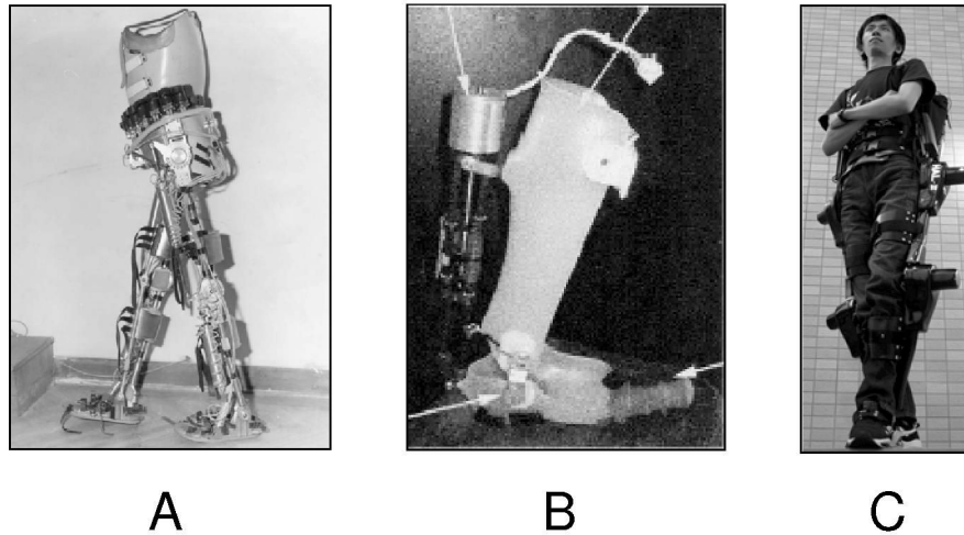
Figure 4. Powered orthoses as assistive technology. A. The exoskeleton developed by Vukobratovic in Yugoslavia in the 1970s. B. Blaya and Herr's powered ankle-foot-orthosis for drop foot correction. C. The hybrid assistive limb (HAL) is currently under development by engineers in the Cybernetics Laboratory at the University of Tsukuba in Japan. Source: A. Vukobratovic et al., Med Biol Eng , January, 1974. Permission to reprint from Peter Peregrinus Ltd. B. Blaya et al., IEEE Trans Neur Sys Eng , 12(1), 24-31, 2004. Permission to reprint from IEEE. C. Original photograph from Prof. Sankai, University of Tsukuba / Cyberdyne Inc. Permission to reprint from Yoshiyuki Sankai, University of Tsukuba. / Cyberdyne Inc.
