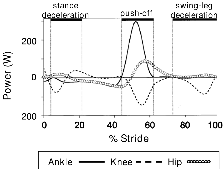
Figure 3. Ankle, knee, and hip joint powers over the stride cycle for normal human walking. Heel strike is at 0% and again at 100%. Toe off occurs at ~ 60%. The majority of the joint power comes from the ankle joint just before toe off. Source: Meinders et al. Scand J Rehab Med 30: 39-46, 1998. Permission to reprint from Taylor and Francis Publishing.
