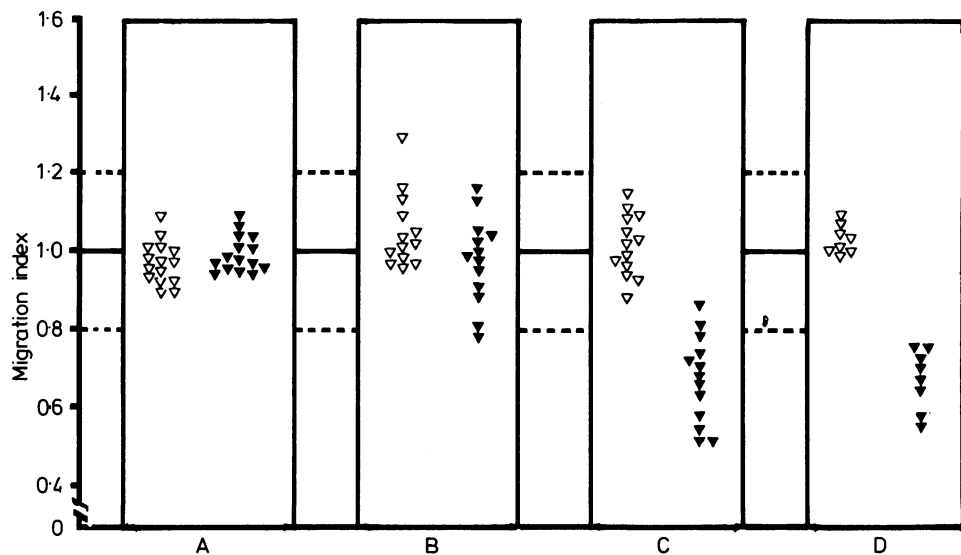
Fig. 2 Indirect LMIF assay: effect of 1 µg/ml alpha-gliadin on the release of LMIF by PBMC into culture supernatant measured by the inhibition of migration of normal leucocytes. \Delta : supernatants from PBMC cultured in the absence of antigen and reconstituted with appropriate concentrations of alpha-gliadin before testing. \blacktriangle : supernatants from PBMC cultured in the presence of alpha-gliadin. A: normal individuals. B: individuals with gastrointestinal disorders other than coeliac disease. C: treated coeliac patients. D: untreated coeliac patients. (Migration indices greater than 1.2 and less than 0.8 represent significant stimulation and depression of migration respectively.)
