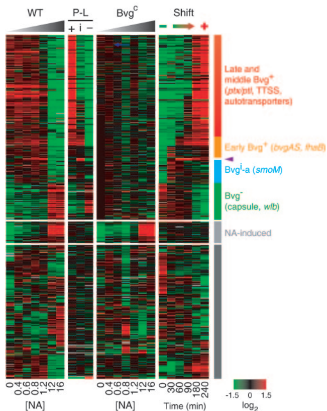
FIG. 4. Patterns of Bvg-regulated gene expression in B. pertussis GMT-1. Data are centered within each experiment. Results obtained with NA modulation and phase-locked strain analysis are shown from Bvg + (left) to Bvg - (right), whereas the phase shift experiment is depicted from Bvg - (left) to Bvg + (right). Rows correspond to array probes, and columns correspond to experiments. +, phase-locked Bvg + ; i, phase-locked Bvg i ; -, phase-locked Bvg - . Red, increased transcript abundance; green, decreased transcript abundance; black, no significant change in transcript abundance; gray, no data. NA concentrations (millimolar) and time elapsed after shift (minutes) are indicated along the bottom. The four major gene expression classes, with some representative loci, and the Bvg-independent NA-induced class are indicated on the right. Purple arrowhead, bipA . The set of genes represented by the gray bar on the right passed filtering criteria but showed no discernible pattern.
