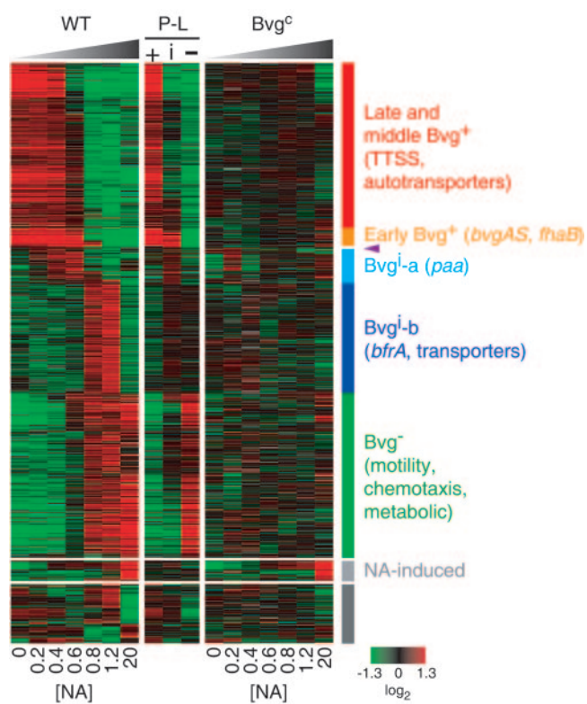
FIG. 3. Patterns of Bvg-regulated gene expression in B. bronchiseptica RB50. Within each experiment, data are centered and shown from Bvg + (left) to Bvg - (right). Rows correspond to array probes, and columns correspond to experiments. +, phase-locked Bvg + ; i, phase-locked Bvg i ; -, phase-locked Bvg - . Red, increased transcript abundance; green, decreased transcript abundance; black, no significant change in transcript abundance; gray, no data. NA concentrations (millimolar) are indicated along the bottom. The five major gene expression classes, with some representative loci, and the Bvg-independent NA-induced class are indicated on the right. Purple arrowhead, bipA . The set of genes represented by the gray bar on the right passed filtering criteria but showed no discernible pattern.
