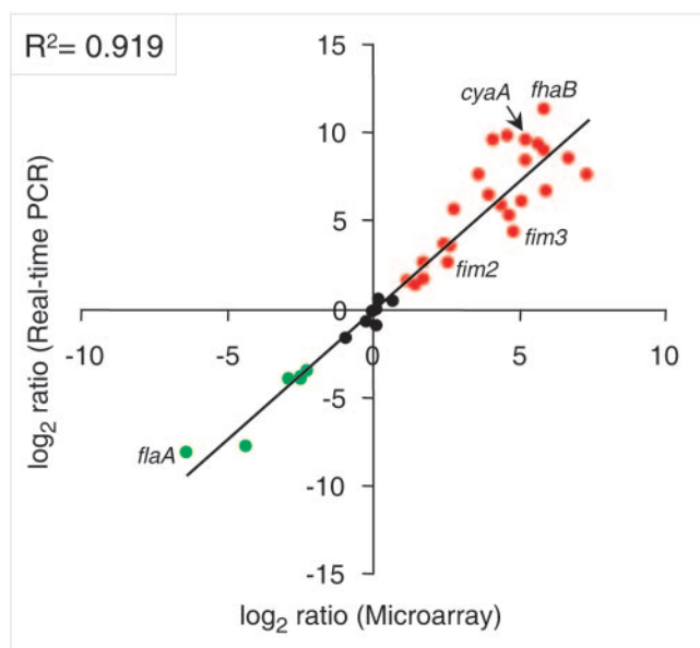
FIG. 2. Validation of B. bronchiseptica microarray data by real-time PCR. Ratios of transcript abundance in RB53 (Bvg + ) versus RB54 (Bvg - ), obtained by microarray analysis (x axis) or real-time PCR (y axis). Red, Bvg activated; green, Bvg repressed. Selected genes are shown for illustrative purposes.
