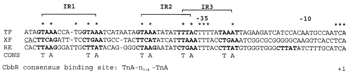
FIG. 1. Alignment of DNA sequences of the cbbR-cbbL intergenic regions of X. flavus (XF), T. ferrooxidans (TF), and R. eutropha (RE). The CbbR binding motif is given below the alignment. *, identical nucleotides. Brackets, positions of LysR motifs. Inverted and direct repeats are in boldface. Positions of the -35 and -10 regions of the cbb promoter are indicated. +1, cbbL transcription start site. The start codon of the cbbR gene of X. flavus is underlined.
