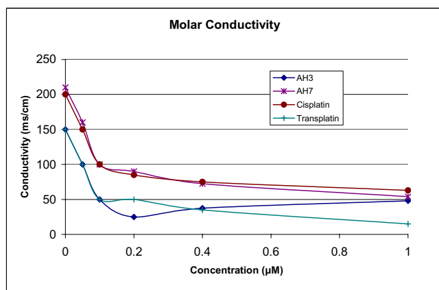
Figure 2 Plots of molar conductivities against concentrations as applied to AH3, AH7, cisplatin and transplatin.
