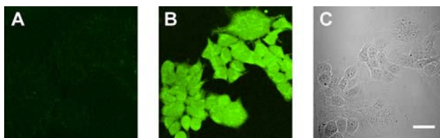
Figure 2. Confocal fluorescence and phase contrast images of live HEK cells. (A) Fluorescence image of HEK cells incubated with 5 \mu\text{M} PF1 for 5 min at 25 ^{\circ}\text{C} . (B) Fluorescence image of PF1-stained HEK cells treated with 100 \mu\text{M} \text{H}_2\text{O}_2 for 5 min at 25 ^{\circ}\text{C} . (C) Brightfield image of live HEK cells after \text{H}_2\text{O}_2 addition to confirm viability. Scale bar = 30 \mu\text{m} .
