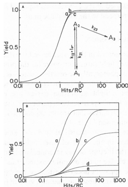
FIGURE 5 Pulse duration dependence of saturation behavior. A , Plots of Eq. 11. All curves calculated with k_{21} = 10^8 s ^{-1} and k_{23} = 5 \times 10^9 s ^{-1} . Pulse duration: curve a , 10^{-6} s; curve b , 10^{-9} s; curve c , 10^{-12} s. A , inset equivalent kinetic scheme for bacterial reaction centers. Extremely rapid reactions that follow the primary photochemical reaction have been incorporated into the photochemical step. A_1 corresponds to P870BpheoUQ, A_2 corresponds to P870 ^+ Bpheo ^- UQ, and A_3 corresponds to P870 ^+ BpheoUQ ^- . B , Plots of Eq. 11. Curve a , calculated with k_{21} = 10^8 s ^{-1} , k_{23} = 5 \times 10^9 s ^{-1} , and pulse duration = 10^{-6} s. Curves b – e , calculated with k_{21} = 10^8 s ^{-1} and k_{23} = 10^7 s ^{-1} . Pulse duration: curve b , 10^{-6} s; curve c , 10^{-7} s; curve d , 10^{-8} s; curve e , 10^{-9} s.
