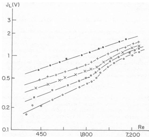
FIGURE 2 Effect on J L as a function of x for a tube obtained by covalent binding to the enzyme running at pH 8. The values of x are the following: (●) 0.3 cm, (+) 1.3 cm, (x) 2.3 cm, (□) 3.3 cm, and (○) 4.3 cm.
