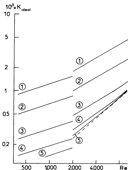
FIGURE 5 Ideal flux computed for different Reynolds numbers and positions along the tube ( r = 0.28 cm, l = 3.5 cm, e = 0.02 cm, D_{LS} = 5 \times 10^{-7} \text{cm}^2/\text{s} , D_{MS} = 2.5 \times 10^{-7} \text{cm}^2/\text{s} ). The dashed line (---) corresponds to a fully developed turbulent flow. x = 50 \mu\text{m} , (1); 300 \mu\text{m} , (2); 0.28 cm, (3); 1.28 cm, (4); and 3.28 cm, (5).
