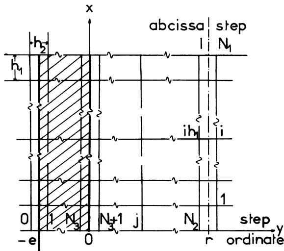
FIGURE 9 Discretization diagram used for the finite difference integration of the partial derivative equations.
