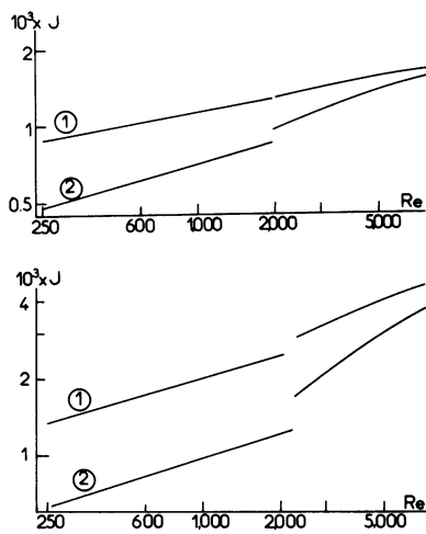
FIGURE 7 Theoretical dependences of J for two values of ET (top, 2.72 \times 10^{-4} cm/s, bottom, 1.36 \times 10^{-3} cm/s) for two positions x = 0.28 , (1), and x = 3.28 cm, (2), as a function of Re .
