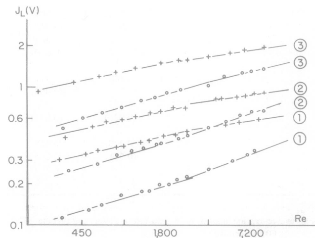
FIGURE 3 Effect of the H_2O_2 bulk concentrations S_1 on the dependence of J_L on Re for a tube obtained by covalent binding to the enzyme and running at pH 8. For each H_2O_2 concentration ( 5.6 \times 10^{-5} , [1], 8.4 \times 10^{-5} [2], and 1.4 \times 10^{-4} M [3]) \log J_L is given at two positions on the tube ( x = 0.3 [+ ] and 3.3 cm [o]).
