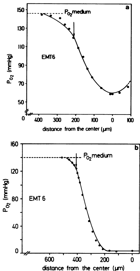
FIGURE 2 Measured P_{O_2} values ( \bullet ) and calculated P_{O_2} profiles ( — ) in multicellular spheroids from EMT6/Ro cells (arrows indicate the spheroid surface). (a) Spheroid without necrosis (diameter: 426 \mu\text{m} ), experiment No. 2/4/81 #4; (b) spheroid with necrosis (diameter: 818 \mu\text{m} ), experiment No. 5/15/81 #16.
