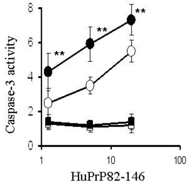
Figure 4 Pre-treatment with IFN- \gamma increases HuPrP82-146-induced caspase-3 activity. Levels of caspase-3 activity in cortical neurons pre-treated with control medium (○), or with 100 ng/ml IFN- \gamma (●) prior to the addition of varying concentrations of HuPrP82-146. Also shown is the caspase-3 activity from neurons pre-treated with control medium (□), or with 100 ng/ml IFN- \gamma (■) and incubated with varying concentrations of HuPrP82-146scrambled. Values shown are the mean percentage fluorescence units from quadruplicate experiments repeated twice (n = 8), \pm SD. ** = Caspase 3 activity significantly greater than untreated neurons incubated with HuPrP82-146 ( p < 0.05 ).
