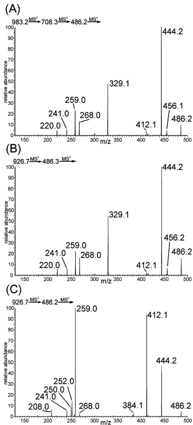
Figure 4. Comparison of (A) an unknown PSM glycan MS 4 spectrum for the ion Hex-HexNAc ( m/z 983→708→486) with the standard spectra of MS n fragments, (B) Gal-β(1-4)-GlcNAc-(1-ene) ( R score, 953), and (C) Gal-β(1-3)-GlcNAc-(1-ene) ( R score, 325) from human milk glycans.
