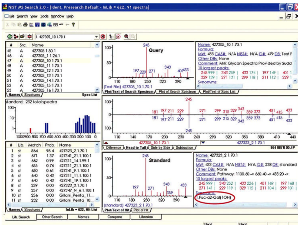
Figure 3. Screen capture of NIST MS tool for FragLib spectral library searching; MS 5 spectrum for Fuc- \alpha -(1-2)-Gal(1-OH) from the human milk glycan lacto- N -difucosylhexaose I (isolated as m/z 1274→834→760→433)(top), compared with the standard spectrum for Fuc- \alpha -(1-2)-Gal(1-OH) stored in FragLib (MS 4 spectrum from lacto- N -fucopentaose I, isolated as m/z 1100→660→433)(bottom).
