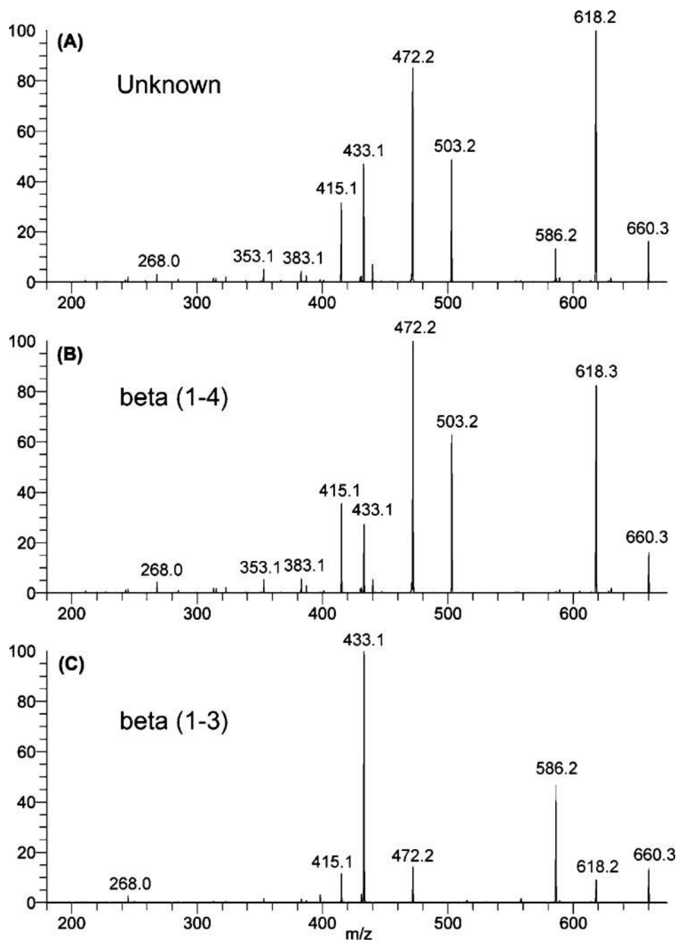
Figure 7. Comparison of (A) an unknown PSM glycan MS 4 spectrum for ion Fuc-Hex-HexNAc ( m/z 1157→882→660) with the standard spectra for (B) Fuc- \alpha (1-2)-Gal- \beta (1-4)-GlcNAc-(1-ene) from PSM glycan ( R score, 838) and (C) Fuc- \alpha (1-2)-Gal- \beta (1-3)-GlcNAc-(1-ene) from human milk glycan ( R score, 623) stored in FragLib.
