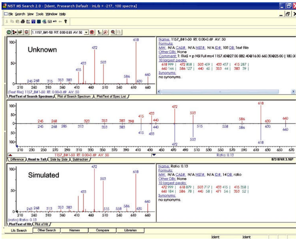
Figure 9. Comparison of the unknown PSM glycan MS 4 spectrum of m/z 1157→882→660 (top) with the simulated standard mixture spectrum (bottom) at the composition percentage of 13% Fuc- \alpha (1-2)-Gal- \beta (1-3)-GlcNAc-(1-ene) and 87% Fuc- \alpha (1-2)-Gal- \beta (1-4)-GlcNAc-(1-ene) ( R score, 874).
