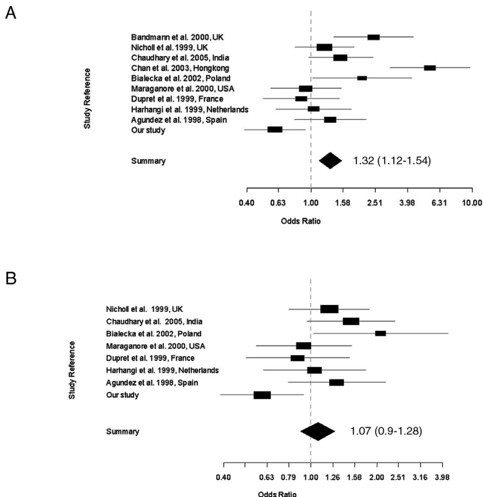
Figure I Meta-analysis of association studies on NAT2 slow acetylators and sporadic Parkinson's disease. The confidence interval for each study is given by a horizontal line, and the point estimate is given by a square whose height is inversely proportional to the standard error of the estimate. The summary odds ratio is drawn as a diamond with horizontal limits at the confidence limits and width inversely proportional to its standard error. (A) : Meta-analysis on 10 studies. Test for heterogeneity \chi^2 (df 9) = 47.71 (p-value 0). The odds ratios are significantly different between the studies. The summary odds ratio (Mantel-Haenszel OR= 1.32, 95% CI, 1.12–1.54) is significantly greater than 1 (p < 0.05). (B) Meta-analysis on 8 studies, excluding studies of Bandmann et al. 2000 and Chan et al. 2003. The odds ratios are not significantly different between studies. Test for heterogeneity \chi^2 (df 7) = 14.28 (p = 0.0464). The summary odds ratio (OR= 1.07, 95% CI, 0.9–1.28) is not significant.
