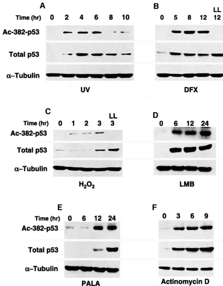
Fig. 1. p53 acetylation induced by multiple p53-activating agents. A549 cells were treated with (A) UV-B (100 J/m 2 ), (C) H 2 O 2 (1 mM) or proteasome inhibitor LLnV (LL, 10 \mu M) for 3 h, (D) LMB (10 ng/ml) or (F) actinomycin D (5 nM). A549 and MCF7 cells (data not shown) were exposed to (B) deferoxamine mesylate (DFX) to mimic hypoxia (100 \mu M) or proteasome inhibitor LLnV (LL, 10 \mu M) for 12 h. WI-38 cells were exposed to (E) PALA (100 \mu M). (A–F) All cells were harvested at the times indicated. All cells contain wild-type p53. Total p53, acetylated p53 and the internal control \alpha -tubulin levels were assessed by western blotting with \alpha -p53 monoclonal antibody (middle panel), \alpha -acetylated p53 (Lys382) (top panel) and \alpha -tubulin monoclonal antibody (bottom panel), respectively. All treatments were carried out without the use of TSA, except for the DFX experiment where 5 \mu M of TSA was added to cells.
