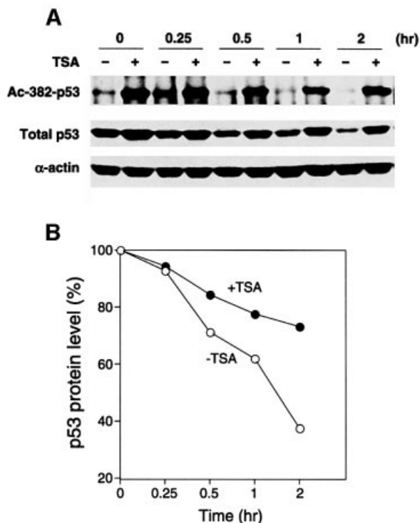
Fig. 6. Inhibition of deacetylase promotes p53 stabilization. (A) A549 cells were exposed to UV-B ( 50 \text{ J/m}^2 ) in the presence (+) or absence (-) of TSA ( 5 \mu\text{M} ). Four hours post-irradiation, cyclohexamide ( 10 \mu\text{g/ml} ) was added to inhibit new p53 protein synthesis (designated 0 h). Cells were harvested at the time-points indicated after cyclohexamide treatment. Acetylated p53 (top panel) and total p53 (middle panel) were determined. Note that total p53 level and acetylation levels are significantly higher in the presence of TSA. As a control, direct western blotting with an \alpha -actin polyclonal antibody also assessed actin levels (lower panel). (B) The band intensity of p53 protein levels was measured by NIH imaging software and calculated against the amount of p53 present at time point 0, which was set at 100%. Results are given in the presence (filled circles) or absence (empty circles) of TSA treatment.
