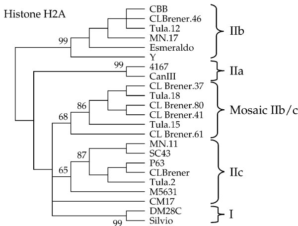
FIGURE 4.—Mosaicism of DTU IIb and IIc alleles within a multicopy locus for heterozygous DTU IId and IIe strains. Neighbor-joining phylogenetic tree of histone H2A intergenic sequences reveals five sequence classes. Mosaic IIb/IIc sequences from CL Brener and Tula strains form their own class.
