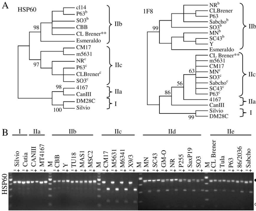
FIGURE 3.—Loci in T. cruzi where DTU IIa/IIc alleles are more similar to DTU IIb. (A) Unrooted neighbor-joining trees of HSP60 and IF8 intergenic sequences reveal four DNA sequence classes. Superscript b or c represent DTU IIb or DTU IIc sequence types, respectively. **, sequence from CL Brener genomic read TCKCA96TR. (B) Agarose gel electrophoresis of PCR-RFLP products from the HSP60 locus of 25 strains. The DNA was stained with ethidium bromide. Size markers (M) are the BRL 1-kb ladders. ● and ○ represent 0.5-kb and 0.1-kb bands, respectively. A SNP at position 125 creates the EcoRV polymorphism in the HSP60 locus (Table 2).
