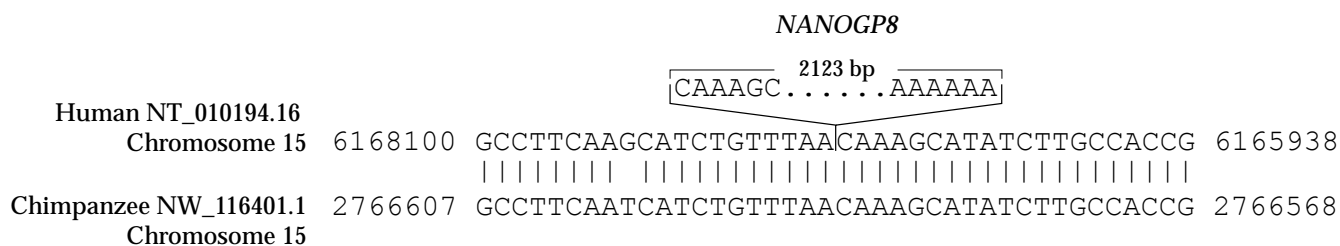
Figure 1 Evidence that the NANOGP8 pseudogene is absent from the chimpanzee genome. Sequences flanking the human NANOGP8 pseudogene on chromosome 15 are present in chromosome 15 of the chimpanzee genome but the pseudogene is absent. Comparison of the human and chimpanzee sequences shows that the NANOGP8 pseudogene inserted itself into human chromosome 15 without duplication of the surrounding sequences.
