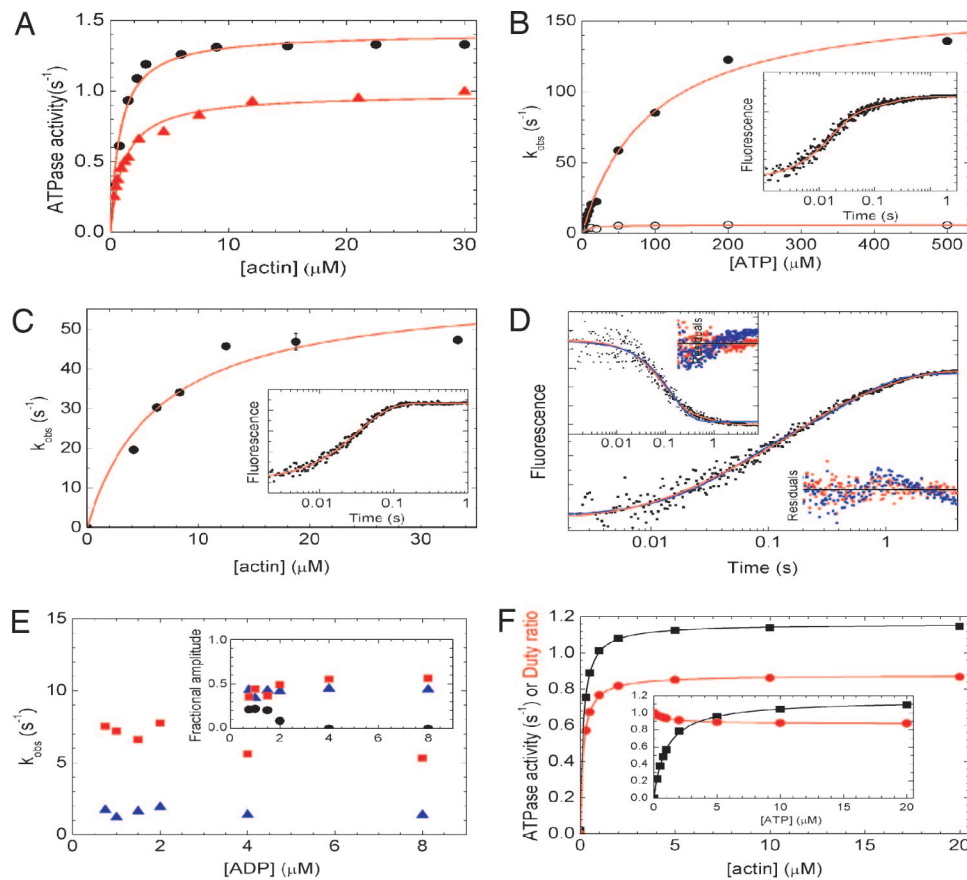
Fig. 4. Kinetic properties of DmVlla. (A) Steady-state actin-activated ATPase activity of DmVlla-S1 and DmVlla-HMM-Zipper. Hyperbolic fit to the data set yielded a maximal ATPase ( V_{max} ) of 1.0 \pm 0.1 \text{ s}^{-1} with half-saturation ( K_{ATPase} ) at 1.1 \pm 0.10 \mu\text{M} actin for DmVlla-S1 (triangles) and V_{max} = 1.4 \pm 0.0 \text{ s}^{-1} with a K_{ATPase} of 0.8 \pm 0.08 \mu\text{M} actin for DmVlla-HMM-Zipper (circles). (B) Observed rate constants ( k_{obs} ) of the fast (filled symbols) and slow (open symbols) phases of ATP-induced dissociation of pyrene-actin-DmVlla-S1 as measured by stopped-flow. The hyperbolic dependence of k_{obs} on [ATP] indicated maximal k_{obs} values of 167 and 5.9 \text{ s}^{-1} for the fast and slow phases, respectively, in the experiment shown. Half-saturation occurred at 93 \mu\text{M} ATP for the fast phase. (B Inset) Trace at 50 \mu\text{M} ATP with k_{obs} values of 59 \text{ s}^{-1} (fractional amplitude: 80%) and 5.5 \text{ s}^{-1} (20%). (C) Observed rate constants ( k_{obs} ) of P_i release in double-mixing stopped-flow experiments in which mVlla-S1 was first mixed with substoichiometric amounts of ATP, incubated for 5 s to obtain the DmVlla-S1-products complex, and then rapidly mixed with various actin concentrations. P_i release was monitored by MDCC-PBP fluorescence (24). The k_{obs} values showed a hyperbolic dependence on actin concentration with a maximum at 61 \text{ s}^{-1} and half-saturation occurring at 6.4 \mu\text{M} actin. (C Inset) Trace at 15 \mu\text{M} actin with a single-exponential k_{obs} of 30 \text{ s}^{-1} . (D) Kinetics of ADP release from actin-DmVlla-S1. Shown is a pyrene-actin fluorescence trace obtained on mixing 0.5 \mu\text{M} pyrene-actin-DmVlla-S1 plus 1 \mu\text{M} ADP with 100 \mu\text{M} ATP in the stopped-flow. A triple-exponential fit (red) to the transient shown yielded k_{obs} of 50.1 (22% fractional amplitude), 7.2 \text{ s}^{-1} (44%), and 1.2 \text{ s}^{-1} (34%). The fastest phase represented ATP-induced dissociation of the nucleotide-free fraction of actin-DmVlla-S1, and the later two phases originated from two populations of actin-DmVlla-S1-ADP (compare Fig. 5). (D Inset) A 2'-deoxy-mant-ADP (dmADP) fluorescence transient recorded upon mixing a premixture of 1 \mu\text{M} actin/ 0.5 \mu\text{M} DmVlla-S1 plus 5 \mu\text{M} dmADP with 1 \text{ mM} ATP in the stopped-flow. Similarly to the pyrene-actin fluorescence records, biphasic ADP release was observed, and a double-exponential fit (red) yielded rate constants of 10.6 \text{ s}^{-1} (67% fractional amplitude) and 1.3 \text{ s}^{-1} (33%). Fits for monophasic ADP release (blue, double-exponential fit in main graph, single exponential in Inset) showed clear systematic deviations from the experimental data (see residual plots; red, biphasic ADP release; blue, monophasic ADP release) in all experiments. Time axes are the same for the data fits and the corresponding residual plots. (E) [ADP] dependence of k_{obs} (main graph) and fractional amplitudes (Inset) of the first (black circles), second (red squares), and third (blue triangles) phase of the transients obtained in experiments described in D. [ k_{obs} values of the first phase are not related to ADP release (see above) and are omitted for clarity.] (F) Steady-state ATPase activity (black) and duty ratio (red) of DmVlla-S1 as obtained in kinetic simulations by using the experimentally determined rate constants of Fig. 5. The duty ratio is defined as the fractional steady-state occupancy of the strongly actin-bound DmVlla-S1 states (underlined in Fig. 5). DmVlla-S1 reaches a maximal steady-state ATPase activity of 1.16 \text{ s}^{-1} and a maximal duty ratio of 0.88 hyperbolically with half-saturation at submicromolar actin concentrations ([ATP] was 1 \text{ mM} in the simulations, in the absence of background ADP). (F Inset) DmVlla-S1 shows a much steeper [ATP]-saturation of its steady-state ATPase activity (half-saturation at 1.0 \mu\text{M} ATP) than other processive myosins ([actin] was 20 \mu\text{M} in the simulations, in the absence of background ADP). At saturating actin and ATP concentrations and in the absence of background ADP, the fractional steady-state occupancy of the various DmVlla-S1 states (Fig. 5) was the following: AM_{closed} , 0.71; AM_{open} , 0.15; AM_{open} , 0.0007; AM_{closed} , 0.0003; AM-T , 0.008; A-MT , negligible; MT , 0.11; MDP , 0.001; AMDP , 0.02. Conditions were 25^\circ\text{C} in 10 \text{ mM} Mops (pH 7.0)/ 2 \text{ mM} \text{MgCl}_2 /0.1 mM EGTA/1 mM ATP/50 mM KCl (10 mM KCl in C).
