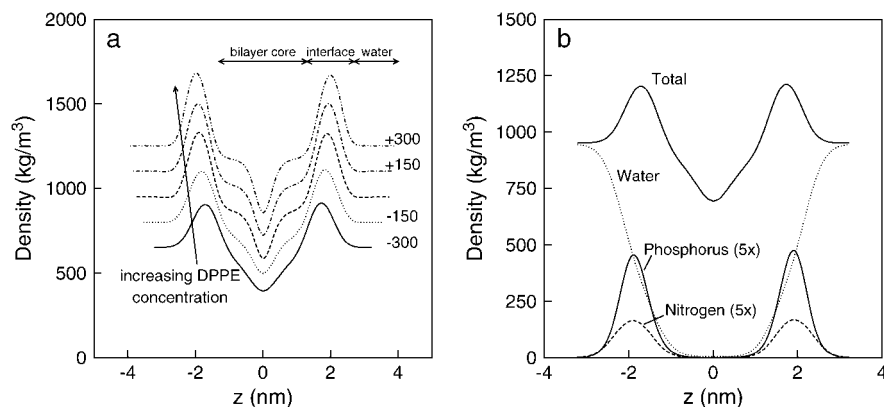
FIGURE 5 (a) Total density profiles of fully hydrated bilayer systems at 350 K. Lines correspond to Lipid-A (solid), Lipid-B (dot), Lipid-C (dash), Lipid-D (dot-dash), and Lipid-E (dot-dot-dash). Numbers are the displacement of the profiles, shifted for clarity. (b) Components density profiles for fully hydrated pure DPPC system at 350 K. Numbers in parentheses are magnification of profiles.
