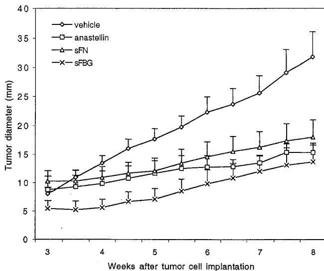
Fig. 3. Inhibition of KRIB osteosarcoma growth by anastellin, sFN, and sFBG. s.c. tumors were grown in nude mice from KRIB osteosarcoma cells. Treatment by i.p. injections of the indicated substances (six mice per treatment group) were started 3 weeks after tumor implantation, repeated twice a week, and continued for 5 weeks. Each injection consisted of 100 \mu g of fibronectin mixed with 300 \mu g of anastellin (sFN), 500 \mu g of fibrinogen mixed with 300 \mu g of anastellin (sFBG), or 600 \mu g of anastellin. Tumor sizes (mean and SEM) in each treatment group (six mice per group) at the indicated time point are shown. The tumors of the mice treated with anastellin, sFN, or sFBG were significantly smaller at the end of the experiment than those of the mice treated with vehicle alone (anastellin, P < 0.01 ; sFN, P < 0.05 ; sFBG, P < 0.01 ).
