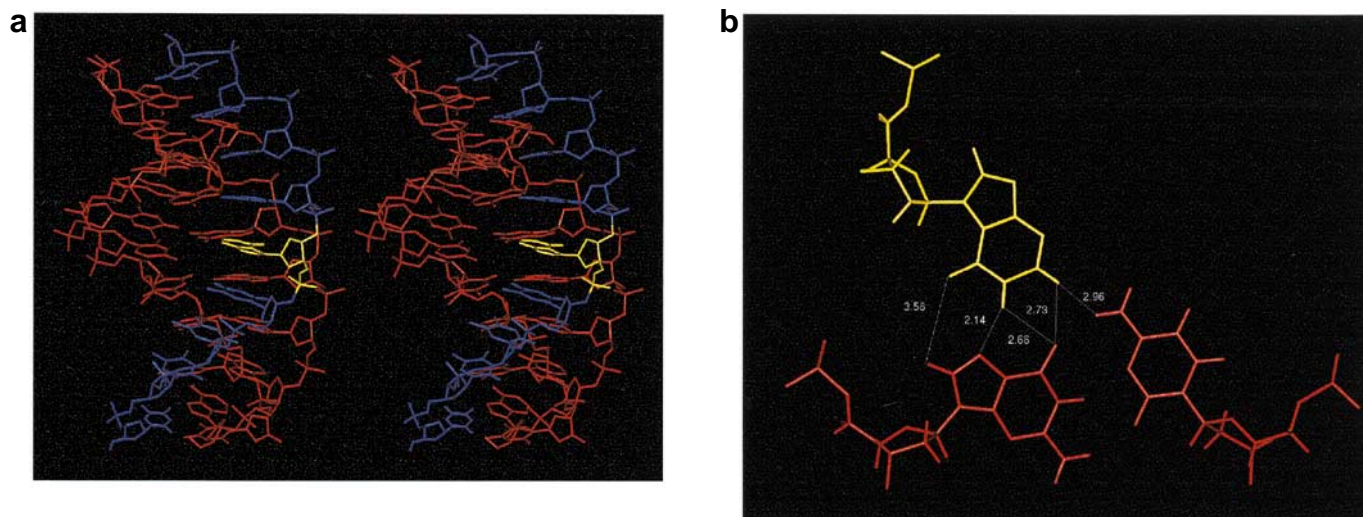
Figure 6. (a) Stereoview of the average structure of the last 50 ps from the 200 ps dynamics simulation of the triplex d(TT^{\text{MeC}^+}T\beta^7HT^{\text{MeC}^+}T^{\text{MeC}^+})\cdot d(AAGAGAGAG)-d(CTCTCTCTT) . The Watson-Crick duplex is colored in red, and the third strand in blue with the \beta^7H residue in yellow. (b) Detailed view of the corresponding \beta^7H\cdot G-C base-triple with selected distances ( \text{\AA} ).
