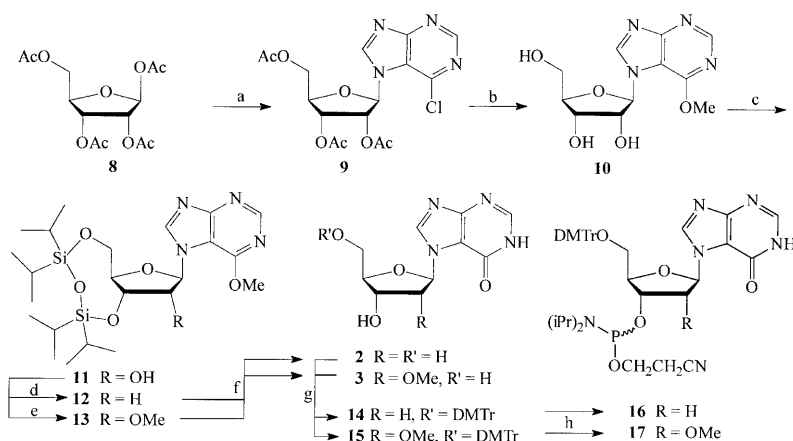
Scheme 2. Reagents and conditions. (a) 6-chloropurine, N,O-bis-trimethylsilylacamide, SnCl 4 , CH 3 CN, 0°C, r.t., 1.5 h, 76%; (b) 0.1 M NaOH in THF:MeOH:H 2 O 5:4:1, 0°C, 1 h, 75%; (c) 1,3-dichloro-1,1,3,3-tetraisopropylidisiloxane, pyridine, r.t., 1.5 h, 79%; (d) (i) p-toluoyl chlorothioformate, DMAP, CH 3 CN, r.t., 16 h, (ii) Bu 3 SnH, AIBN, toluene, 75°C, 2 h, 82%; (e) NaH, MeI, DMF, -25°C, 2.5 h, 82%; (f) 1 M NaOH in THF:MeOH:H 2 O 5:4:1, 70°C, 5.5 h, 81% ( 2 ), 89% ( 3 ); (g) (MeO) 2 TrCl, pyridine r.t., 2 h, 54% ( 14 ), 73% ( 15 ); (h) (NCCH 2 CH 2 O)[(iPr) 2 N]P(=O)Cl, EtN(iPr) 2 , THF, 1 h, 63% ( 17 ), 64% ( 16 ).
