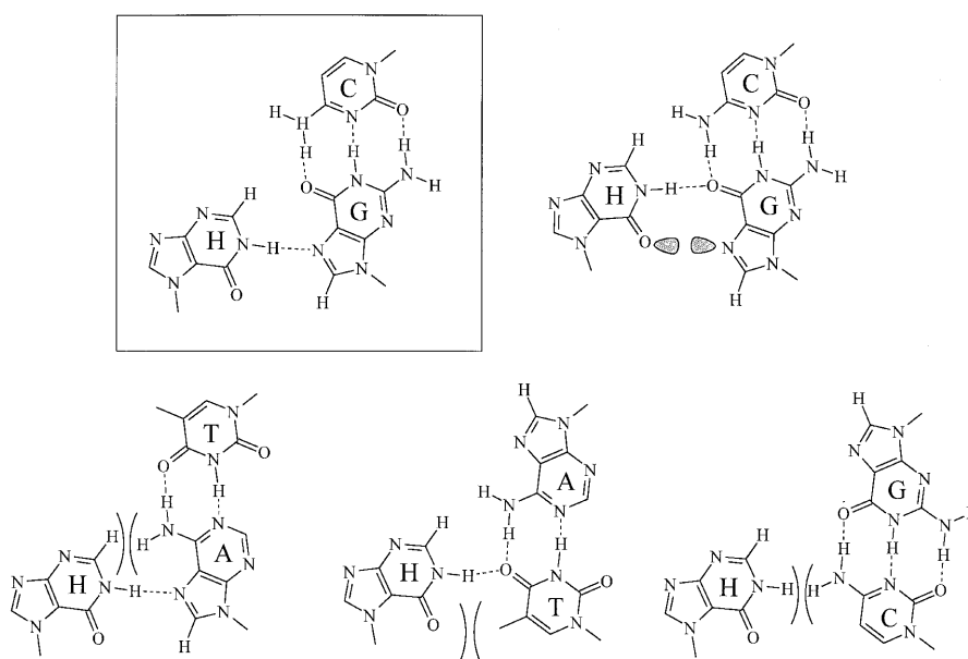
Figure 5. Base arrangements of the \text{N}^7 -hypoxanthine residues with the natural DNA Watson-Crick base pairs.
