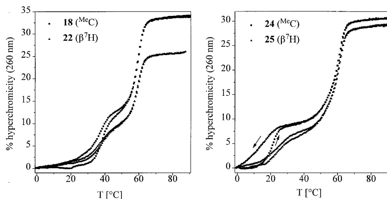
Figure 4. UV-melting curves (heating and cooling cycle) of oligonucleotides 18 , 22 , 24 and 25 (concentration = 1.2–1.6 \mu\text{M} in 10 mM Na-cacodylate, 100 mM NaCl, 0.25 mM spermine, pH 7.0) with the corresponding DNA target 21mers shown in Figure 2.
