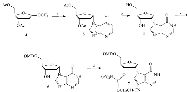
Scheme 1. Reagents and conditions. (a) 6-chloropurine, HMDS, TMSCl, SnCl 4 , MeCN, r.t., 3 h, 51% (+ N 9 -mixture \alpha,\beta 2.5:1, 37%); (b) 1 M NaOH in THF:MeOH:H 2 O 5:4:1, 0–65°C, 5h, 75%; (c) (MeO) 2 TrCl, pyridine r.t., 3 h, 68%; (d) (NCCCH 2 CH 2 O)((iPr) 2 N]P(=O)Cl, EtN(iPr) 2 , THF, r.t., 1.5 h, 69%.
