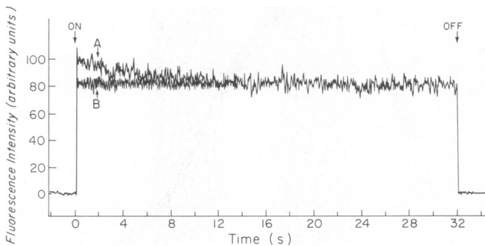
FIGURE 5 Fluorescence intensity of light-adapted purple membrane as a function of time at -196^{\circ}\text{C} . (A) After preillumination with 640 nm light. (B) After preillumination with 590 nm light. Measuring optical bandwidth, 9.9 nm; excitation optical bandwidth, 6.6 nm; \lambda excitation, 590 nm with 590-nm interference filter in the exciting beam; \lambda measuring, 680 nm with CS 2-61 filter before the analyzing monochromator.
