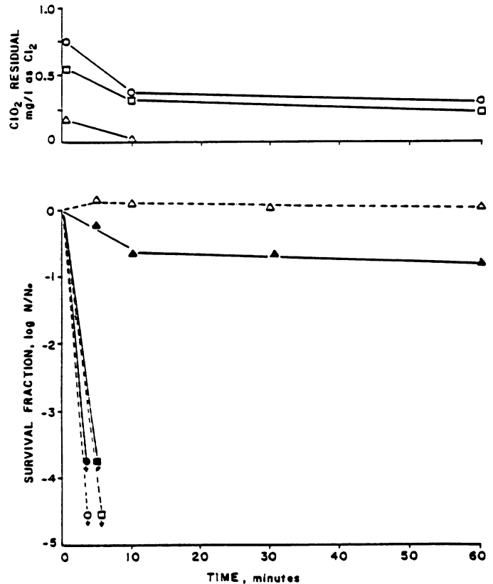
FIGURE 5. Inactivation of f2 virus (solid symbols) and E. coli B (open symbols) by 0.17 (△), 0.55 (□) and 0.75 (○) initial chlorine dioxide (ClO₂) residual as available chlorine in the presence of 1% autoclaved raw sewage. All of pH 7.0, 25°C.
