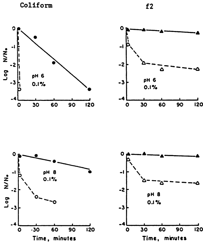
FIGURE 4. Inactivation of coliform (○) and f2 (△) in the presence of 0.1% sewage with an approximate initial chlorine residual of 0.3 mg/L at pH 6.0 and 8.0. Open symbols: initial free chlorine residual, average of four trials; closed symbols: initial combined chlorine residual, average of five trials.
