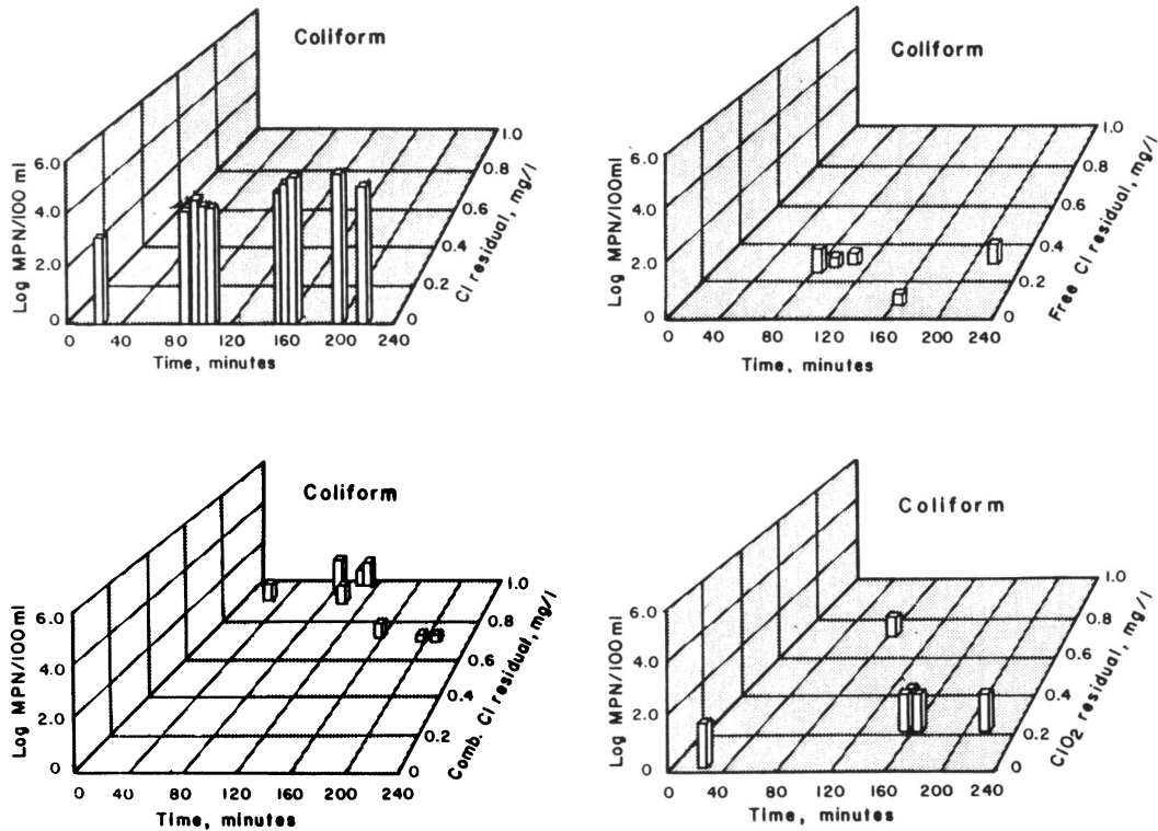
FIGURE 10. Level of coliform at the tap in the test distribution system with no residual disinfectant and an initial 1.04 mg/L free chlorine, 1.08 mg/L combined chlorine and 0.95 mg/L chlorine dioxide residual. Temperature 13–17°C; pH 7.3–7.7.
