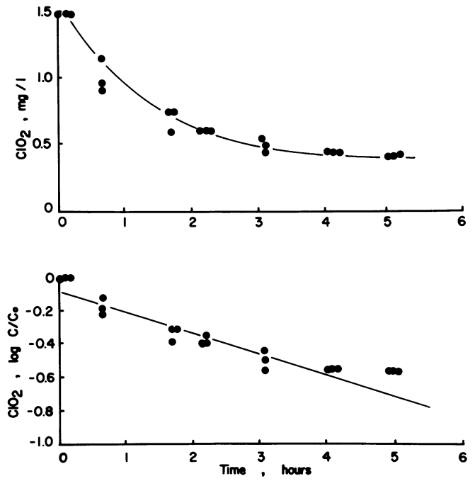
FIGURE 16. Stability of chlorine dioxide at three stations in the test distribution system under static conditions. Temperature 22°C; pH 7.7.
