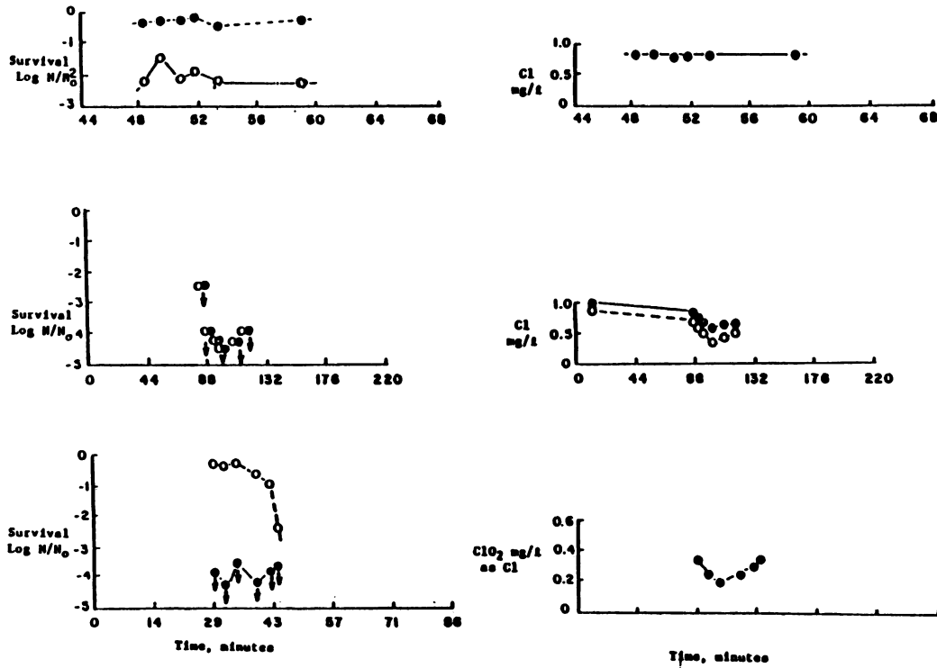
FIGURE 9. Survival of the microorganisms in the raw sewage challenge and different disinfectant residuals. For initial combined chlorine: (○) coliform; (●) f2, temperature approximately 15–20°C, pH 8.2 (top panel); for free chlorine, temperature 14°C, pH 7.6 (middle panel); and for chlorine dioxide, temperature 10°C, pH 7.5 (bottom panel).
