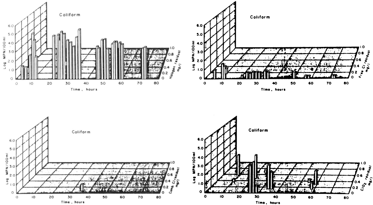
FIGURE 12. Level of coliform at the tap in the test water distribution system with no residual disinfectant and an initial 1.0 mg/L free chlorine, combined chlorine, and chlorine dioxide residual. Temperature 19–22°C; pH 7.3–8.2.
