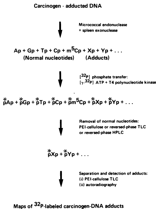
FIGURE 1. The basic features of ^{32}\text{P} -postlabeling assay for carcinogen-adducted DNA. The ^{32}\text{P} -assay involves four steps: digestion of DNA, ^{32}\text{P} -labeling of the digestion products, removal of ^{32}\text{P} -labeled nonadduct components, and TLC mapping of the [ ^{32}\text{P} ]adducts. Asterisks indicate the position of the ^{32}\text{P} -label. Purification of adducted nucleotides derived from carcinogens having two or more aromatic rings (e.g., BP, DMBA, DBC, and ABP) is accomplished by PEI-cellulose TLC (13–15), while for adducts carrying a single aromatic ring (e.g., alkenylbenzenes and sterigmatocystin) or a bulky nonaromatic ring (e.g., MMC), octadecyl silane reversed-phase TLC is preferred (16,18,19,21).
