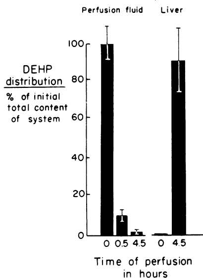
FIGURE 7. DEHP distribution in the isolated, perfused rat liver.
