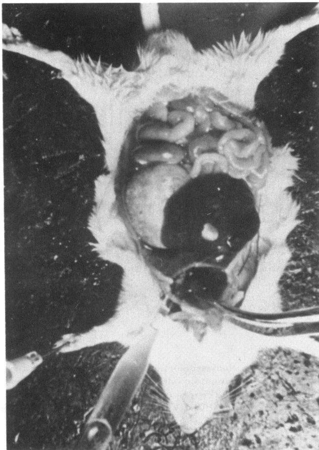
FIGURE 1. Pathological responses to 4-ipomeanol in the mouse 24 hr after a 35 mg/kg dose, IP: (left) massive pleural effusion (fluid in pipet); (right) section showing prominent intra-alveolar edema.
