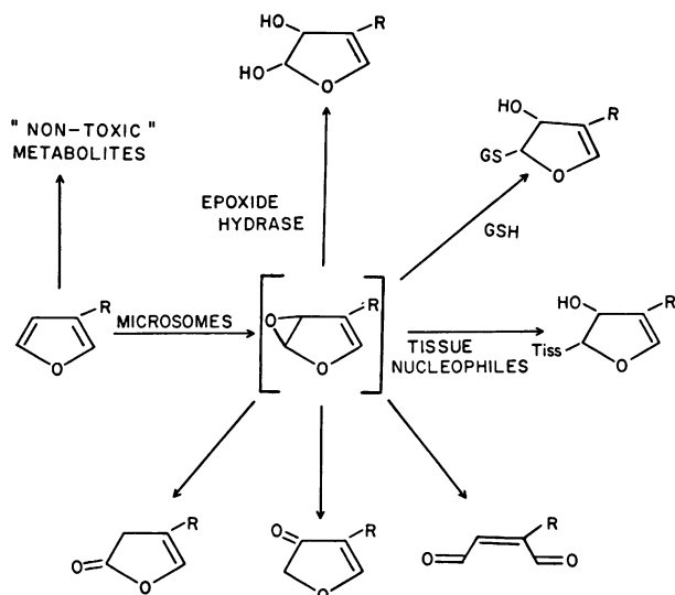
FIGURE 5. Possible pathways for toxication and detoxication of 4-ipomeanol.
