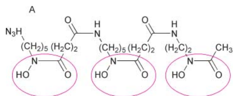
Desferrioxamine B
