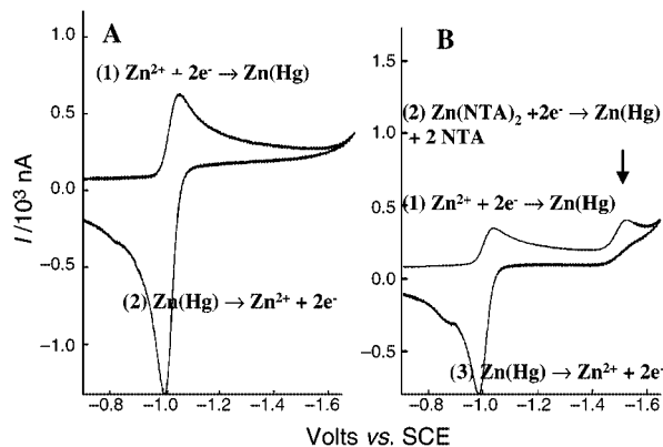
Fig. 1 Cyclic voltammograms of (A) 100 \mu M inorganic Zn in seawater and (B) 100 \mu M Zn with 50 \mu M NTA. Peak 2 is due to the reduction of Zn in ZnNTA_2 . Peak 1 in each CV is due to inorganic Zn reduction and peak 3 is due to the oxidation of Zn in the amalgam.
