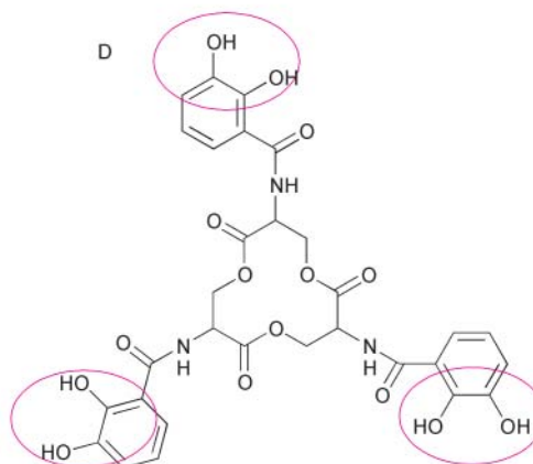
Enterobactin
