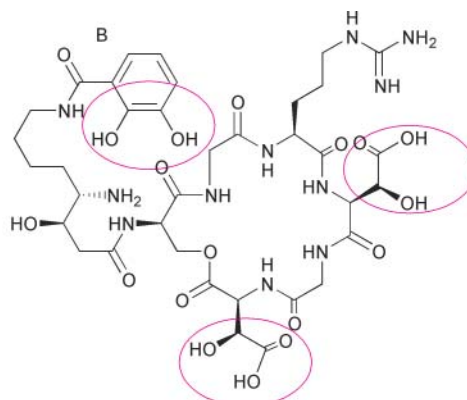
Alterobactin A
