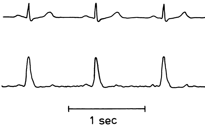
Fig. 2: Comparison of electrocardiograms (Standard lead 2) registered Mingograf minor 3 with paper speed of 50 \text{ mm}\cdot\text{s}^{-1} (upper curve) and with EMG analyser (Me-10 RI) recorded with Animex Recorder at the same speed (lower curve).
