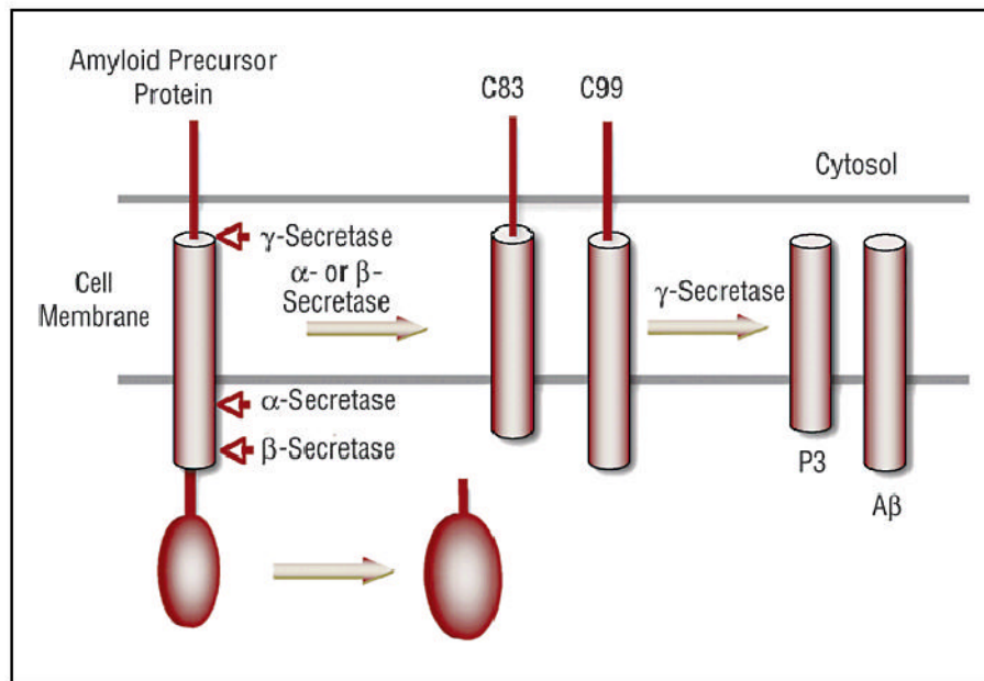
Figure 1. Amyloid precursor protein processing. Amyloid precursor protein is processed by \alpha - or \beta -secretase to products C83 or C99, respectively. \gamma -Secretase processes C83 and C99 to P3 and A\beta , respectively. \beta Amyloid then can polymerize to form oligomers (A\beta)_n in the amyloid plaque.
