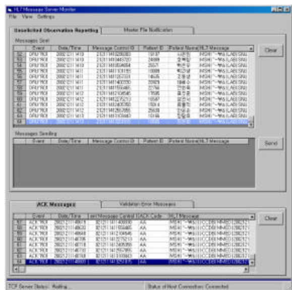
Figure 7: User Interface for monitoring the HMS
