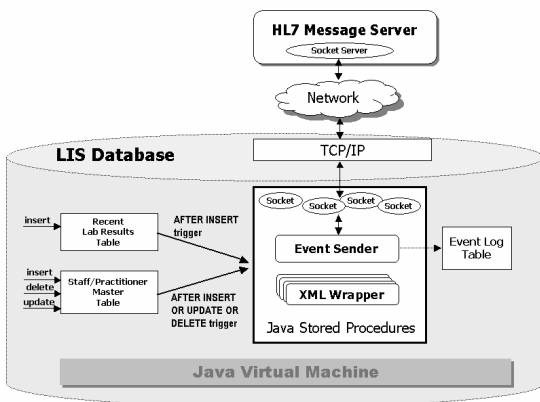
Figure 4: Architecture for transferring real-time data
