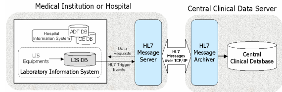
Figure 2: HL7 Message-based Standard Interface Architecture
