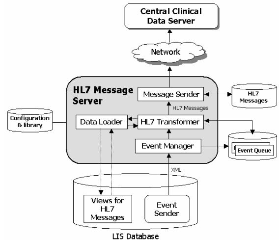
Figure 6: Architecture of the HL7 Message Server
