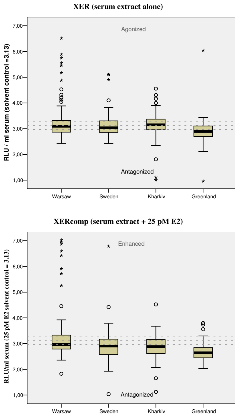
Figure 1 The xenoestrogenic CALUX activity of study groups. (A) Agonistic activity of serum extracts alone (XER) and (B) competitive XER activity upon coexposure with 25 pM E2 (EC 40 ) (median, quartiles (25% and 75%) and extreme variables). For the Swedish study group an extreme agonistic (A) RLU value of 12.02 was determined (not shown). The reference line of the respective solvent controls ± SD (3.13 ± 0.16) are given as dotted lines.
