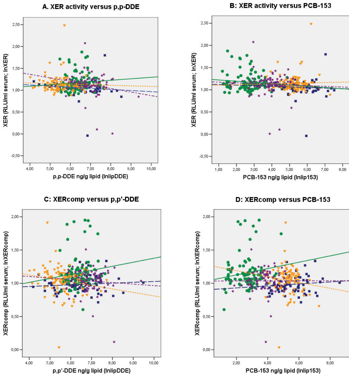
Figure 2 Schematic illustration of xenoestrogenic activities related to the POP markers. Xenoestrogenic (XER) and competitive XER (XERcomp) serum activities related to CB-153 and p,p'-DDE levels for the four country based study groups as a relation between (A) XER and p,p'-DDE, (B) XER and CB-153, (C) XERcomp and p,p'-DDE, and (d) XERcomp and CB-153. The values are given as ln transformed data. Greenland: ■--- ; Warsaw: ●— ; Sweden: ▼- - - ; Kharkiv: *- - -
