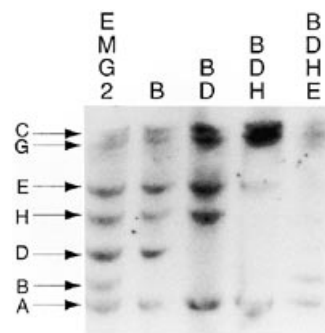
Figure 2. Autoradiogram of a Pst I and Bam HI double digest of chromosomal DNA from deletion strains B, BD, BDH, (B)DHE and base strain EMG2. The genomic blot was hybridized with Oligo 5S-M (complementary to the deleted nucleotide sequence in 5S rRNA genes). The seven operons (A, B, D, G, H, E and C) are identified with their specific restriction fragments.
