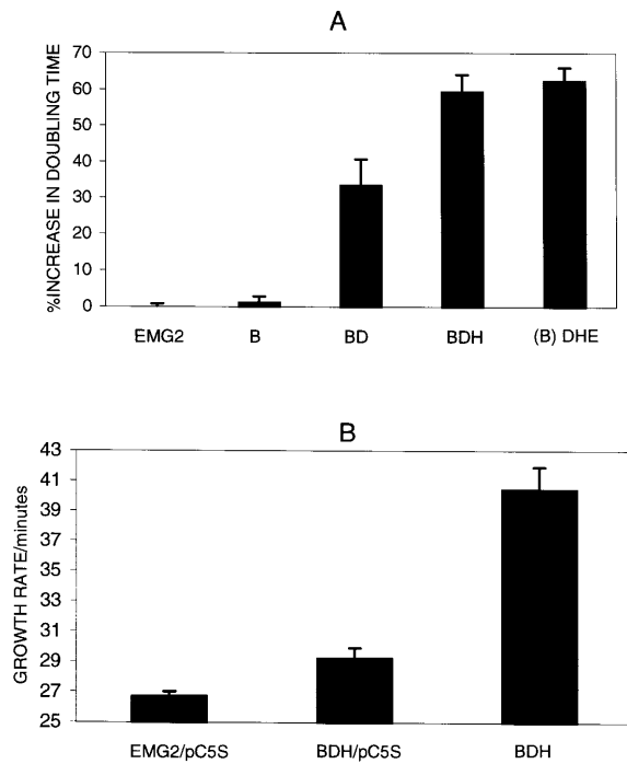
Figure 4. (A) Doubling times of 5S rRNA deletion strains B, BD, BDH and (B)DHE presented as percent increase in doubling time relative to the base strain EMG2 ( 27.6 \pm 0.6 min). (B) Doubling times of the base strain EMG2 grown with the compensatory plasmid pC5S (representing the maximum growth rate), strain BDH (representing the minimum growth rate) and strain BDH with compensatory plasmid pC5S. Values represent the average growth rate for multiple trials. The standard deviation between the trials is shown as an error bar.
