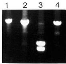
Figure 3. Evidence for reacquisition of a 5S rRNA gene in operon B of strain (B)DHE by a gene conversion event. An ethidium bromide stained agarose gel of DNA from selected strains using primers 0 and B. Primer 0 amplifies from any of the operons, whereas primer B is specific for operon B. Lane 1, EMG2 digested with Xba I; lane 2, BDH undigested; lane 3, BDH digested with Xba I; lane 4, (B)DHE digested with Xba I.
