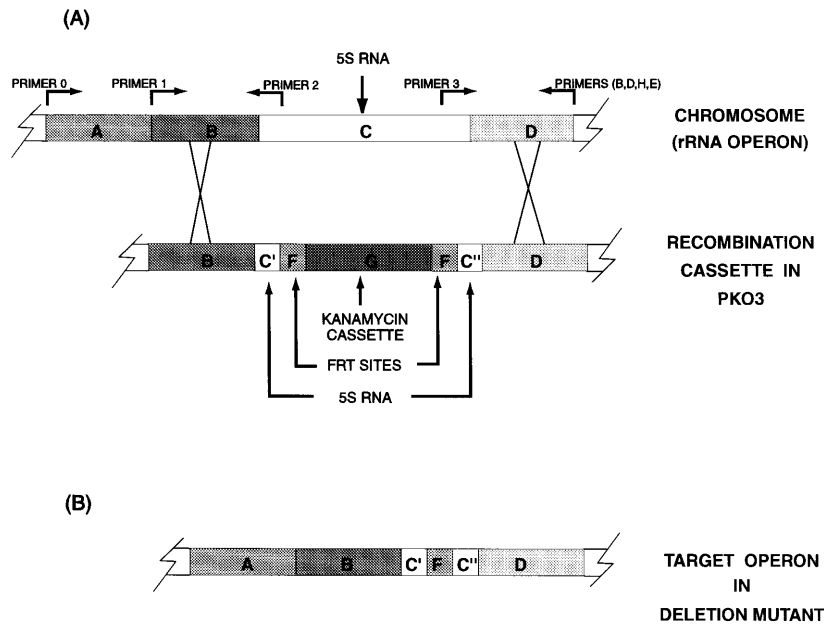
Figure 1. (A) The double crossover event between the recombination cassette in pKO3-(B, D, H or E) and the corresponding chromosomal operon in E. coli strain EMG2 is illustrated. (B) Composition of a 5S rRNA deleted rRNA operon after Flp-mediated excision of the kanamycin gene. Letters represent different DNA regions. A, B and D are regions of 468, 531 and 517 bp, respectively, which flank the 5S rRNA. Region C is 120 bp, region G is ~1500 bp and region F is ~75 bp. Regions C' and C'' are 18 and 20 bp in length, respectively, and represent the terminal 18 and 20 nt of the 5S rRNA gene that are complementary to primers 2 and 3. FRT is a DNA sequence recognized by Flp recombinase resulting in the loss of one FRT site and the entire DNA between the two FRT sites.
