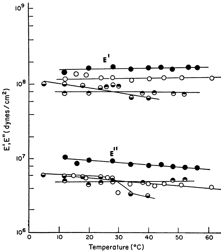
FIGURE 4 Dynamic modulus E' and dynamic loss modulus E'' of type C cut strips of bovine cornea as a function of temperature at ●—● 110; ○—○ 35; ●—● 11; and ○—○ 3.5 Hz frequencies.
