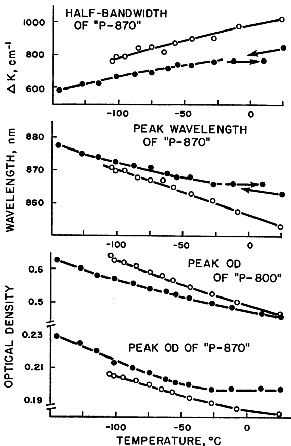
FIGURE 13 Parameters in the absorption spectra of reaction centers measured at various temperatures. Filled circles: dried film as in curve A of Fig. 6. Open circles: reaction centers in glycerol-H 2 O as in Fig. 9. The half-bandwidth of P-870 was measured as follows: the wavelength was recorded at the absorption maximum and at the position of half-maximum OD on the long wave side of the peak. These wavelengths were converted to wave number (reciprocal of wavelength, centimeters -1 ) and their difference was doubled to yield \Delta k .
