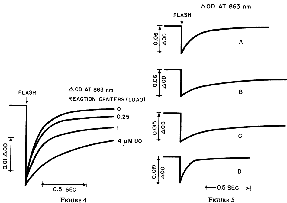
FIGURE 4 Flash-induced \Delta OD at 863 nm in reaction centers with varying concentrations of added UQ (coenzyme Q_8 ) as shown. Reaction centers made with LDAO were suspended to 0.9 \mu M in 0.01 M Tris-Cl, pH 7.5, with 0.05% LDAO.
