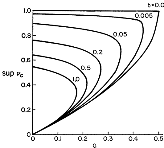
FIGURE 3 Pulse height \sup_x v_c(z) versus a for various positive values of b , determined from Eq. 11 for 0 \leq z \leq z_1 . For b = 0 , the upper branch corresponds to a transition waveform given by Eq. 54 for which \sup v_c = v_c(\infty) = 1 . The lower branch for b = 0 corresponds to a standing pulse given by Eq. 56, for which \sup_x v_c(x) = v_c(x_1/2) .
