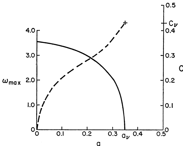
FIGURE 10 Maximum frequency, \omega_{\max}(a, b) = \max_{c, c_s} [\sup_{P > P_{\min}} (cP^{-1})] , of periodic wave trains shown solid as a function of a , for b = 0.05 . Propagation speed of the wave with \omega_{\max}(a, b) plotted (dashed) versus a for b = 0.05 .
