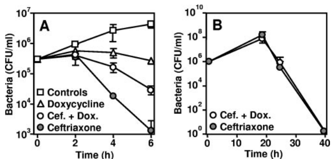
FIG. 3. Interaction of ceftriaxone and doxycycline in vitro and in vivo. (A) In vitro time kill curves for S. pneumoniae . The bacteriostatic antibiotic doxycycline ( 1 \times \text{MIC} ) inhibited growth of pneumococci. The bactericidal antibiotic ceftriaxone ( 4 \times \text{MIC} ) rapidly killed the pneumococci. The combination of doxycycline ( 1 \times \text{MIC} ) and ceftriaxone ( 4 \times \text{MIC} ) (Cef. + Dox.) exhibited in vitro antagonism. (B) Bacterial CSF titers in vivo at 0, 18, 24, and 40 h after infection with live pneumococci. At 24 h (6 h after the initiation of antibiotic treatment) combined therapy with doxycycline (30 mg/kg) and ceftriaxone (100 mg/kg) (Cef. + Dox.) and therapy with ceftriaxone (100 mg/kg) alone did not result in significantly different bacterial titers in the CSF ( 8.0 \times 10^5 \pm 15.0 \times 10^5 CFU/ml [ n = 23 ] and 3.2 \times 10^5 \pm 6.7 \times 10^5 CFU/ml [ n = 21 ], respectively [not significantly different]). At 40 h after infection, CSF samples from all animals were sterile.
