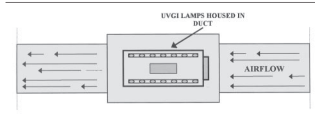
Figure 4. Placement of UVGI lamps in air ductwork (section view) with UVGI lamps placed perpendicular to the airflow
