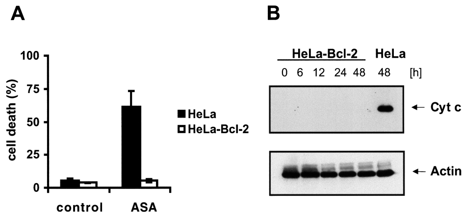
Figure 6. Overexpression of Bcl-2 prevented aspirin-induced cytochrome c release and apoptosis. (A) FACS analysis and (B) Western blotting of cytosolic extracts after treatment with 5 mM aspirin for the indicated time period. The percentage of annexin V positive cells was measured by FACS analysis after treatment with aspirin for 48 hours.
