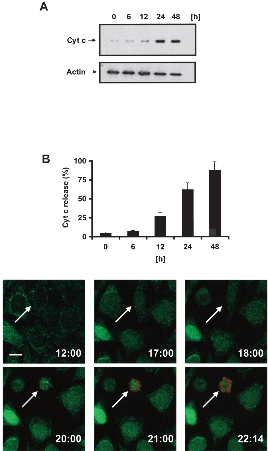
Figure 4. Aspirin induces the release of cytochrome c from HeLa cells. HeLa-Cc-GFP cells were treated with 5 mM ASA and analyzed for cytochrome c release by means of (A) Western blot with cytochrome c antibody, (B) FACS analysis (CLAMI assay), or (C) multicolor time-lapse confocal microscopy. Cytochrome c-GFP (green) moves from a mitochondrial staining pattern to a cytoplasmic distribution. Loss of plasma membrane integrity was detected by uptake of propidium iodide (red). The arrow indicates a cytochrome c-releasing cell; the number at the bottom right of each frame represents the time after treatment with aspirin. Images were taken with a \times 60 objective and zoomed 1.8 times. Scale bar = 15 \mu m.
