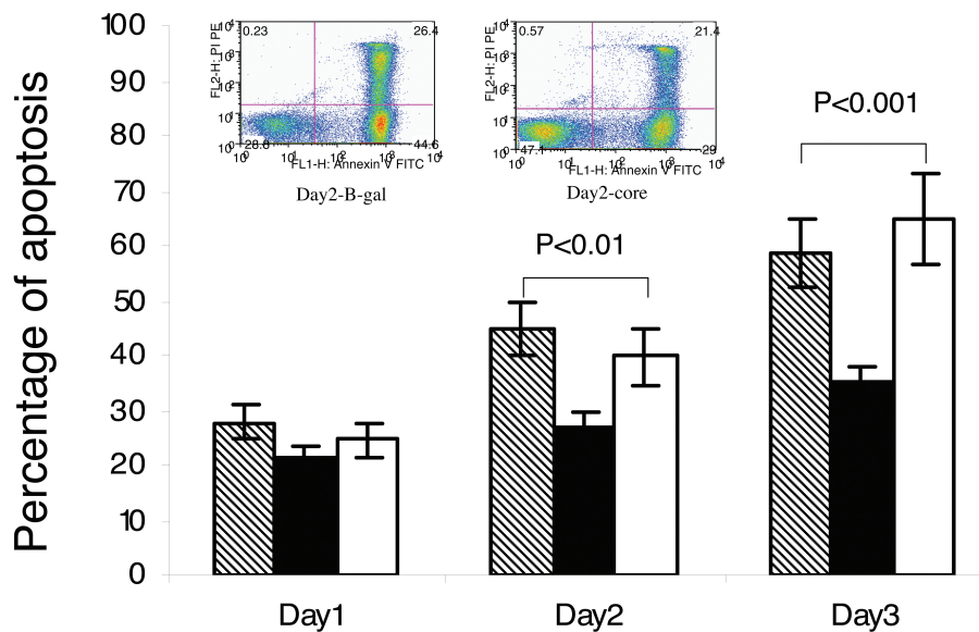
Figure 2. Percentage of apoptotic B cells during 3-day viral infection with adenovirus harboring \beta -galactosidase (striped bar), HCV core (solid bar), and HCV NS3 (open bar). Data were calculated with average value of duplicate experiments in B cells derived from two donors. Inset represents FACS analysis of annexin V- and IP-stained B cells 2 days after infection of Ade- \beta -gal (left) and Ade-core (right).
