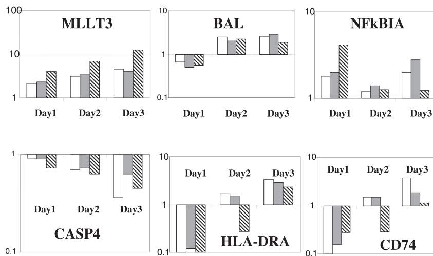
Figure 4. Comparison of fold changes in gene expression of six representative genes between duplicate quantitative RT-PCRs after normalization with 18S RNA (open and gray bars) vs. the mean value from two microarray experiments (hatched bar) during 3-day viral infection. The fold change is expressed on a logarithmic scale. If a gene expression value is greater than 1, the gene is upregulated; if less than 1, the gene is downregulated.
