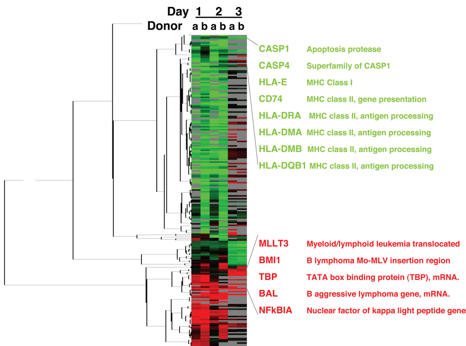
Figure 3. Hierarchical analyses of 216 differentially expressed genes from duplicate experiments in B cells derived from two donors (A and B) as described in Figure 1. The upregulated genes are shown in red and the downregulated ones in green. The representative genes are listed.
