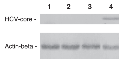
Figure 1. Western blot analysis for HCV core protein expression in human B cells 48 h after introduction with no adenovirus (lane 1) and with adenovirus harboring \beta -galactosidase (lane 2), HCV NS3 (lane 3), and HCV core (lane 4). Relative amount of total protein of each sample was normalized by \beta -actin.
