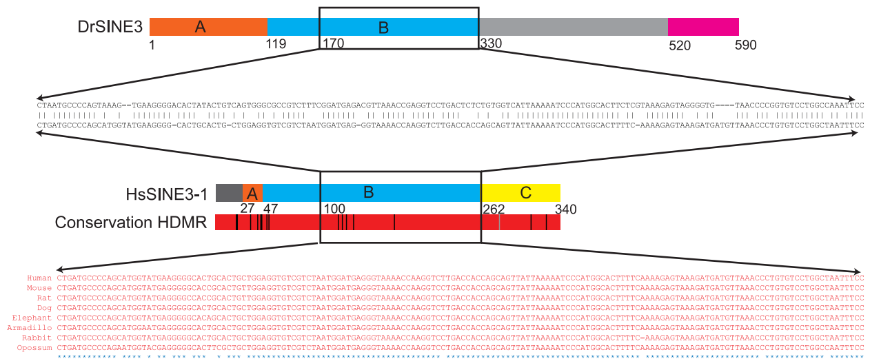
Fig. 1. Comparison of the zebrafish DrSINE3 transposable element and HsSINE3-1 as well as the orthologous conservation of HsSINE3-1 across various mammals. Related portions are shown in the same color. Most of the similarity between the human sequence and DrSINE3 lies within the central core region (shown in blue and labeled “B”); the best aligning portion of 162 bp in humans is indicated by the rectangle and shown as a pairwise alignment. For conservation across HDMR, colors are as follows: red, identical 4-way; black, nonidentical 4-way; gray, <4 bases align. The corresponding orthologous sequence in seven other mammals is shown as a multiple alignment in red.
