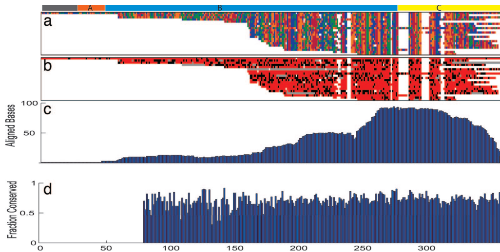
Fig. 2. A multiple alignment of the top 20 human instances most similar to HsSINE3-1 was carried out. (a) The multiple alignment by color-coding bases (A, blue; G, green; T, red; C, orange). (b) The orthologous conservation profile across HDMR (perfect four-way identity, red; four bases aligned imperfectly, black; fewer than four bases aligning, gray). All 124 members of HsSINE3 were aligned to the reference instance HsSINE3-1. (c) How often a base was mapped to a given position along the reference. (d) The rate of perfect HDMR conservation along the reference for mapped human bases.
