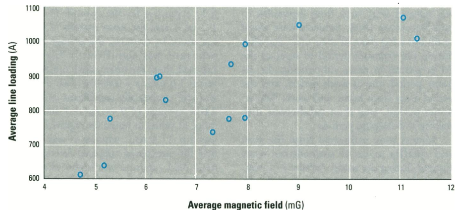
Figure 1. Correlation between the average magnetic field personal exposure at home and the average current loading in the power line during the measurement period for the exposed group (n = 14); r = 0.80; p = 0.001.
