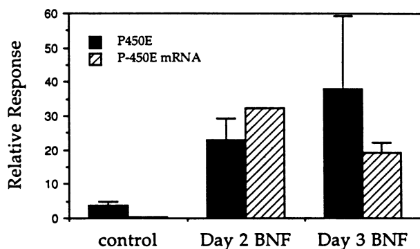
FIGURE 2. Induction of cytochrome P-450E protein and mRNA in scup. Scup were treated IP at day 0 with 20 mg/kg BNF in corn oil, and microsomes and RNA fractions were prepared and analyzed as described elsewhere (32).
