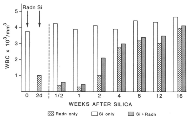
FIGURE 1. Numbers of white blood cells (WBC) in the radiation-only, silica-only, and combined treatment groups to 16 weeks. Control value is shown at time 0.
