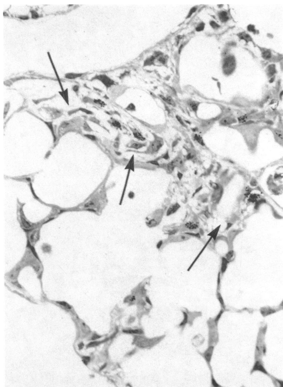
FIGURE 3. Lung section 12 weeks after whole-body irradiation only, showing alveolar walls thickened by fibrosis (arrows). \times 750 .
