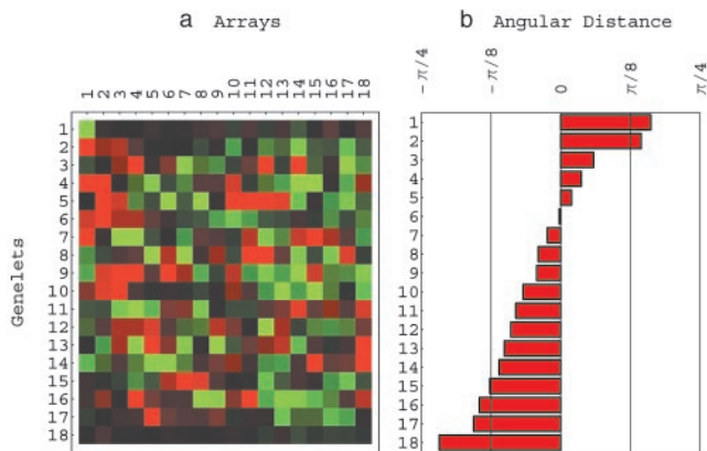
Fig. 1. Yeast and human genelets. (a) Raster display of \hat{\lambda}^{-1} , the expression of 18 genelets in 18 yeast and human arrays simultaneously, centered at their array-invariant levels. (b) Bar chart of the angular distances showing \langle\gamma_1\rangle and \langle\gamma_2\rangle highly significant in the yeast data relative to the human data, \langle\gamma_3\rangle , \langle\gamma_4\rangle , \langle\gamma_5\rangle , \langle\gamma_6\rangle , \langle\gamma_{14}\rangle , \langle\gamma_{15}\rangle , and \langle\gamma_{16}\rangle almost equally significant in both data sets and \langle\gamma_{17}\rangle and \langle\gamma_{18}\rangle highly significant in the human data relative to the yeast data. All other genelets are significant in neither the yeast data nor the human data (see Appendix).
