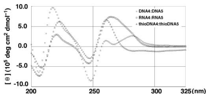
Figure 5. CD spectra of duplexes consist of ON4:ON5.
