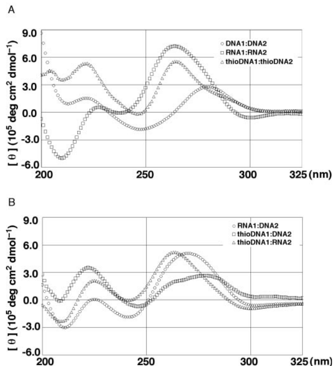
Figure 3. CD spectra of duplexes consist of ON1:ON2.
