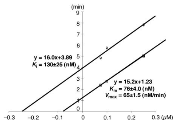
Figure 8. Hanes-Woolf plots of RNase V_1 and RNA1:RNA2 without (square) and with thioDNA3 (circle). Errors reflect standard deviation from three independent experiments.
