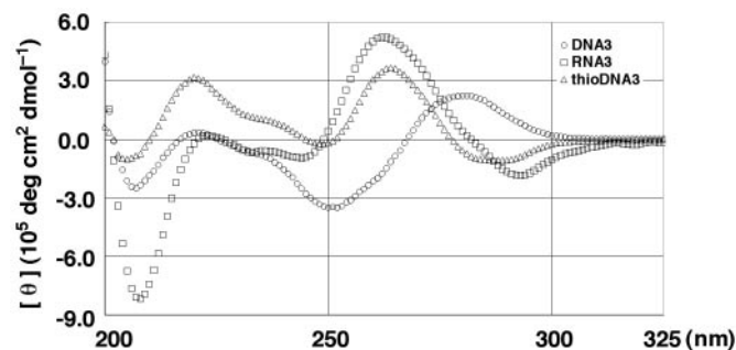
Figure 4. CD spectra of self-complementary duplexes consist of ON3.
