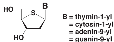
Figure 1. Structure of 2'-deoxy-4'-thionucleosides.
