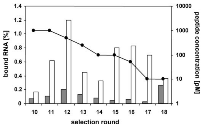
Figure 4. Progress of manual selection rounds (10–18) using the short library. The histogram shows the progress of the manual in vitro selection carried out with the short library starting from round 10. The black circles indicate the peptide target concentration offered in the respective selection round. In each selection round equal amounts of radio-labelled RNA were incubated with the respective peptide concentrations and with pure selection matrix as a control in order to verify the specific enrichment of binding sequences versus unspecific binding. The fraction of RNA specifically binding to the target peptide (white columns) is compared to the fraction of RNA that unspecifically binds to the selection matrix (grey columns).
