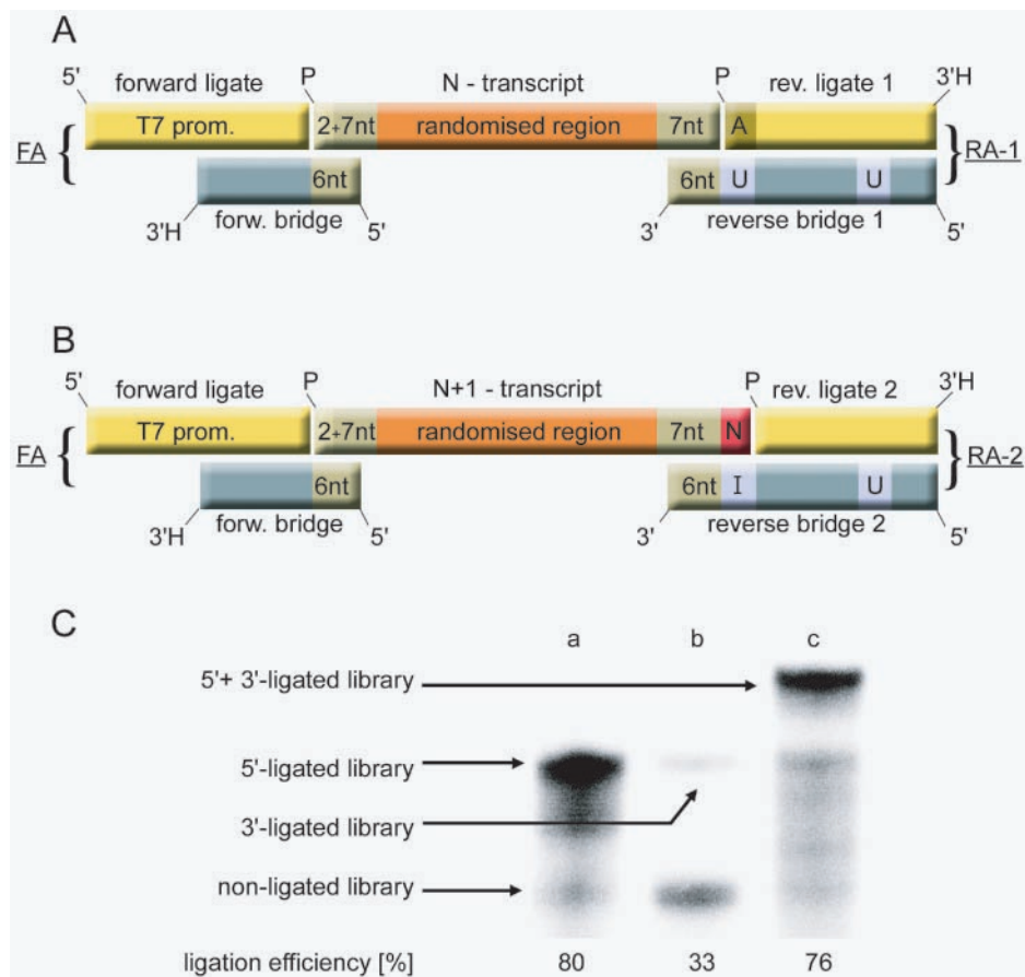
Figure 3. Template-directed ligation of the short RNA library. The cartoon (A and B) presents the structural designs of the short RNA library (N- and N+1-transcripts) and the double-stranded adapters which consist each of a ligate and a bridge. The randomized region (34 nt) is flanked by seven nucleotides that can form base pairs (see Figure 1), where upon the 5' end carries two additional fixed nucleotides. Six nucleotides at both ends of the library serve as hybridization sites for the forward bridge and the two reverse bridges. The uridines (U) and the inosine (I) in the reverse bridge 1 (A) and 2 (B), respectively, introduce the alkaline fission sites into the primer binding site. The forward bridge, the reverse ligates 1 and 2 additionally contain a 3'-terminal 2',3'-dideoxynucleotide (3'-H) to prevent mispriming during PCR. Up to 50% of all transcripts are N+1-transcripts (B) that contain a non-coded nucleotide at the 3' end. In order to ligate primer binding sites to these molecules as well, the reverse adapter 2 was designed. It comprises the reverse ligate 2 i.e. 1 nt shorter at its 5' end than ligate 1, and reverse bridge 2 that offers the universal base inosine (I) for hybridization to the non-coded nucleotide in the N+1 position of the transcript. The autoradiogram (C) exemplarily shows the results of the template-directed ligation. While ligation yield of the forward adapter to the 5' end of the RNA molecules was acceptable (lane a), the ligation of the two reverse adapters 1 and 2 to the 3' end of the library was with ~33% quite insufficient (lane b). However, in the case that both forward and reverse adapters are present in equimolar amounts at the same time, the overall ligation yield was markedly improved (lane c). FA: forward adapter; RA-1: reverse adapter 1; RA-2: reverse adapter 2; forw: forward; rev: reverse; prom: promoter; nt: nucleotides.
