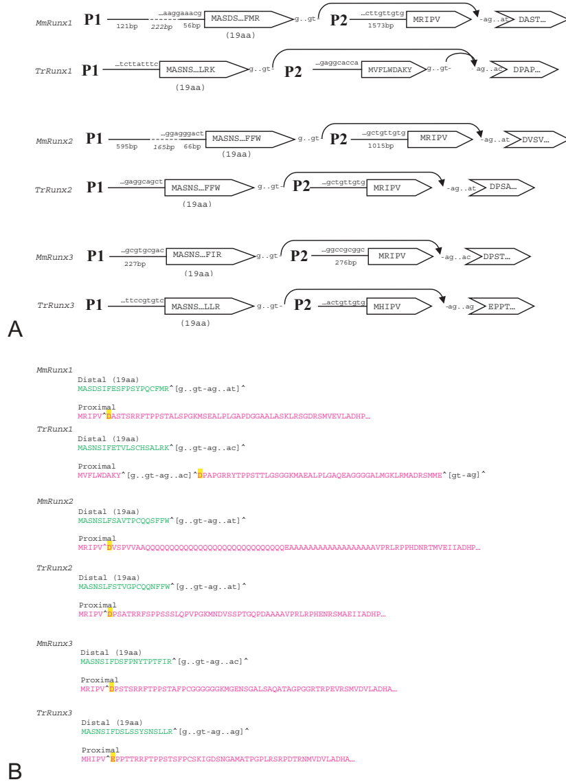
Figure 4 Alternative transcripts and N-termini produced by transcription from proximal and distal promoters of vertebrate runx genes. (A) Diagram of alternative transcripts from distal (P1) and proximal (P2) promoters in vertebrate Runx genes. Solid lines represent untranslated regions of exons, while dashed lines represent introns. TrRunx1 distal transcript is theoretical and based on its similarities to other distal transcripts (i.e., its open reading frame begins with a sequence encoding MASNS), location (~14 kb from proximal transcript) and size (19 aa). TrRunx2 and TrRunx3 transcripts from P1 were derived from similarities to MmRunx2 and Danio rerio runtb , respectively. TrRunx2 was recently published [11]. M. musculus distal transcripts were gathered from Genebank entries and verified with publications (see Supplemental Table 1). Note: Unlike all of the other vertebrate Runx genes in our collection, TrRunx1 transcript from P2 has a small exon (encoding 9 amino acids) followed by a 1 kb intron (see also B, below, and 3). This small exon splices into the same location within the downstream coding sequence as does the exon from the distal transcript. (B) Alternative N-terminal amino acid sequences of various vertebrate Runx genes analysed in our survey. N-termini from the distal promoters are shown in green, while the N-termini from the proximal promoters are shown in red. The aspartate or glutamate to which the N-terminal sequences from the distal promoter are joined are highlighted in yellow. The positions and nucleotides at the termini of introns are indicated in lower case.
