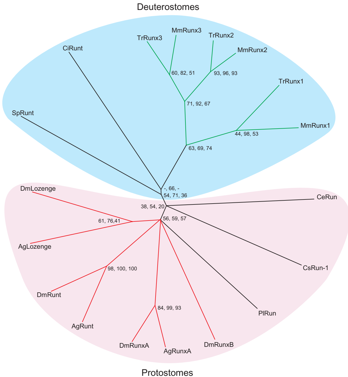
Figure 3 Phylogenetic tree of the Runx protein family. Maximum likelihood tree calculated with the assumption of a molecular clock from the multiple amino acid sequence alignment shown in Figure 2. The numbers at each node are the bootstrap support values obtained by maximum likelihood (no molecular clock assumed), neighbour joining, and maximum parsimony, in that order. The dashes (-) by the branch leading to the Ciona gene ( CiRunt ) indicate that the maximum likelihood and maximum parsimony methods did not support that node (these methods each place CiRunt on a branch with TrRunx1 , with support values of 50 and 52, respectively). Branches with unresolved topology were collapsed. Coloured branches are used to highlight the vertebrate lineage (green) and the insect lineage (red). The shading highlights the deuterostome (blue) and protostome (pink) representatives in the sample. Abbreviations for species names are the same as in Figures 1 and 2.
