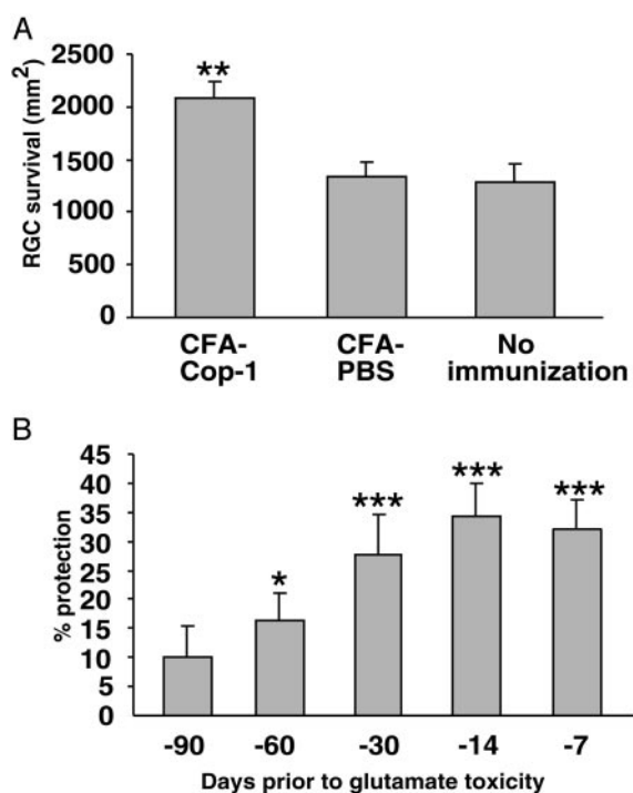
Fig. 2. Cop-1 vaccination protects RGCs against glutamate toxicity. (A) C57BL/6J mice ( n = 6) were immunized with Cop-1 emulsified in CFA. Ten days later the mice were subjected to unilateral intraocular injection of toxic amounts of glutamate (200 nmol). As controls, we used a group of mice injected with glutamate only ( n = 7) and a group of mice ( n = 8) that were immunized with PBS in CFA 10 days before being exposed to glutamate. Three days after their exposure to glutamate, the RGCs were retrogradely labeled. Retinas were excised 1 week after their exposure to glutamate. RGC survival was assessed by counting the labeled cells, and is expressed as mean ± SEM per mm 2 . A two-tailed Student's t test was used for statistical analysis. (B) C57BL/6J mice were immunized with Cop-1 in CFA at the indicated time points before receiving unilateral intraocular injections of toxic amounts of glutamate (200 nmol). After an additional 7 days they were killed, their retinas were excised, and RGC survival was assessed. Mice that received only glutamate were used as controls. Protection is expressed in terms of RGC survival, calculated as a percentage of RGC survival in control mice.
