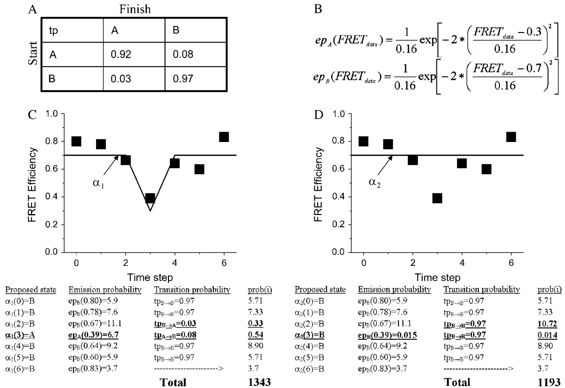
FIGURE 2 Evaluating probabilities in a hidden Markov model. (A) The transition probability matrix gives the likelihood that a molecule in one state will transit to another in a single time step. (B) Emission probability functions ( ep_A , ep_B ) define the probability of observing a FRET value FRET_{data} when in a given conformation (A or B). The emission probability functions and the transition probability matrix shown are for a known two-state system with underlying FRET values 0.3 and 0.7 (state A and state B, respectively) and a width in the distribution of 0.16, similar to the system depicted in Fig. 1. (C) Generated data (squares) are plotted together with a proposed sequence of states ( \alpha_1(i) ). By using the parameters from A and B, we can evaluate the probability that the proposed sequence could generate the observed data for each time point and then take their product to find the total. (D) The same is done for an alternative proposed sequence of states ( \alpha_2(i) ) with differences highlighted in bold and underlining. By comparing the total probabilities of 1343 for \alpha_1(i) to that of 1193 for \alpha_2(i) we deduce that a transition likely took place at time step 3.
