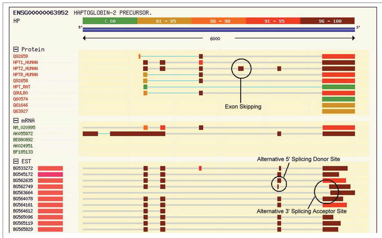
Figure 2 An example ProSplicer analysis showing how the three types of alternative splicing event will be displayed.
