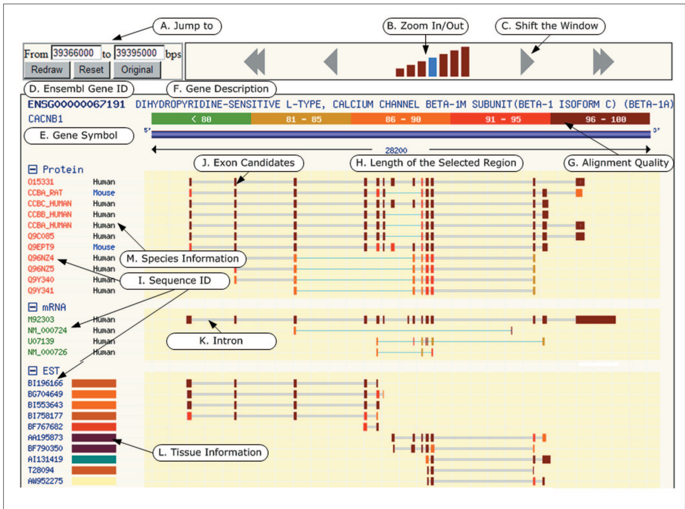
Figure 4 The 'detailed view' graphical interface in ProSplicer.
