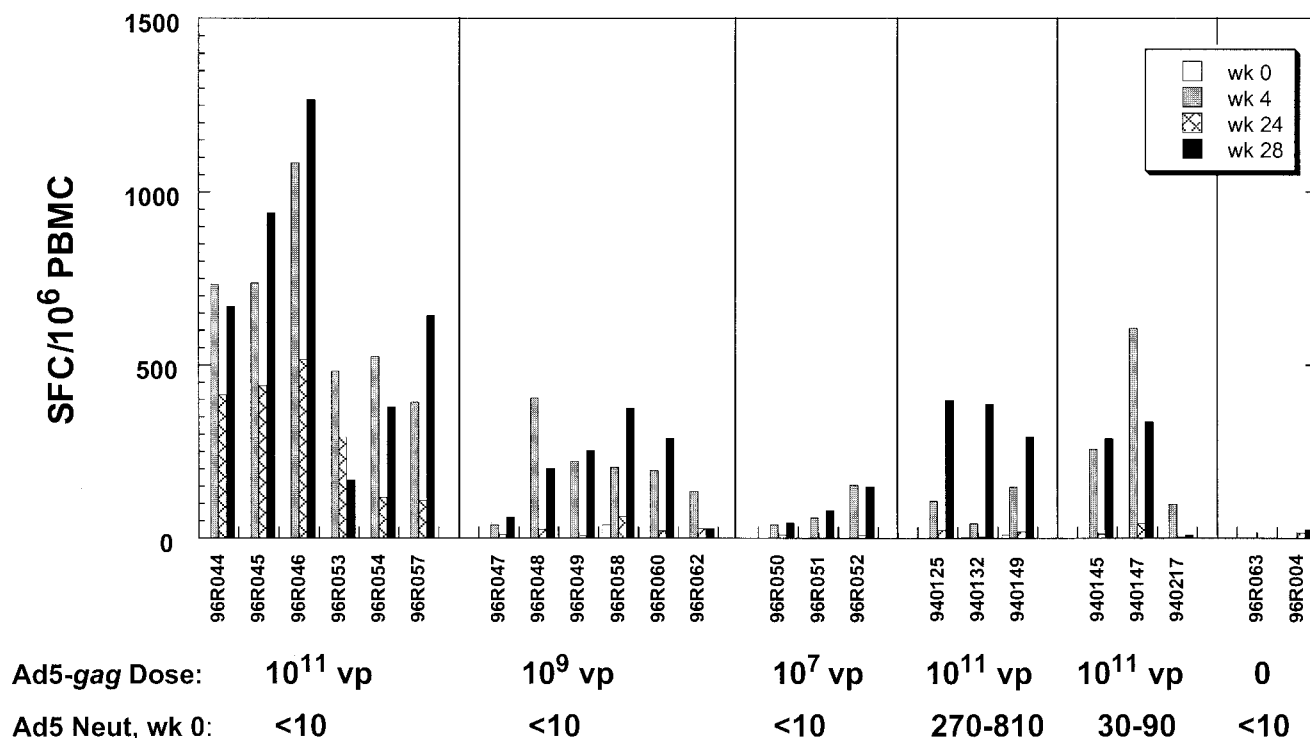
FIG. 1. Frequencies of Gag-specific IFN- \gamma -secreting cells from monkeys immunized with Ad5-gag. These values are expressed as the number of SFC per 10^6 PBMCs. Naïve monkeys (adenovirus type 5 neutralization (neut) titers < 10 ) were immunized with various doses of Ad5-gag at weeks 0 and 24. Monkeys that were pretreated with one or three 10^{10} viral particle (vp) doses of non-Gag-encoding adenovirus type 5 virus (producing neutralization titers of \approx 30 to 90 and \approx 270 to 810 , respectively, at the time of the first Ad5-gag injection) were immunized with 10^{11} viral particles of Ad5-gag at weeks 0 and 24. PBMCs collected at weeks 0, 4, 24, and 28 were incubated in the absence (mock) or presence of the HIV-1 Gag peptide pool, and the mock-corrected response levels are shown here for each monkey. Mock-treated background responses averaged 3 SFC per 10^6 PBMCs (standard deviation, \approx 5 SFC per 10^6 PBMCs).
