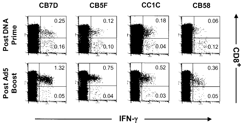
FIG. 7. Intracellular IFN-γ staining of PBMCs from a representative cohort of macaques immunized with three doses of V1jns-gag formulated with CRL1005-based adjuvant (weeks 0, 4, and 8) followed by 10 7 viral particles of Ad5-gag boost (week 24). Samples were collected at week 10 (postprime) and week 28 (postboost). Shown are CD3 + lymphocytes following incubation with the HIV-1 Gag peptide pool that were characterized for CD8 + staining and IFN-γ production. For all samples, intracellular IFN-γ production in the absence of the peptide pool was minimal (data not shown). Numbers reflect the percentage of CD3 + lymphocytes that were CD8 + IFN-γ + (upper right quadrant) or CD8 + IFN-γ - (lower right quadrant) after subtraction of the mock levels.
