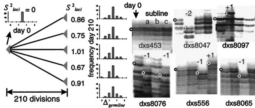
Fig. 2. A single HCT 116 cell was isolated, grown, and subsequently split into different sublines. After 190–332 days, single clones were isolated from each subclone, were expanded for 20 more divisions, and were typed at 24 MS loci (autoradiographs from three 210-day-old sublines and six loci are illustrated). Relative to germline (open circles or the allele size of the original clone), subline alleles are randomly the same, or larger or smaller (filled circles). The distribution of these changes ( \Delta_{germline} ) and their estimated variances ( S^2_{loci} ) are small compared with human tumors (compare with Fig. 3). Variation between alleles at a single locus is minimal because only 20 divisions occurred during terminal expansions ( S^2_{alleles} \approx 0 ). This experiment mimics five simulated trials with a history of 210 divisions since loss of MMR and a terminal clonal expansion of 20 exponential divisions (see Fig. 1c). The experimental S^2_{loci} values are consistent with the simulations (see triangles in the graph of Fig. 1c).
