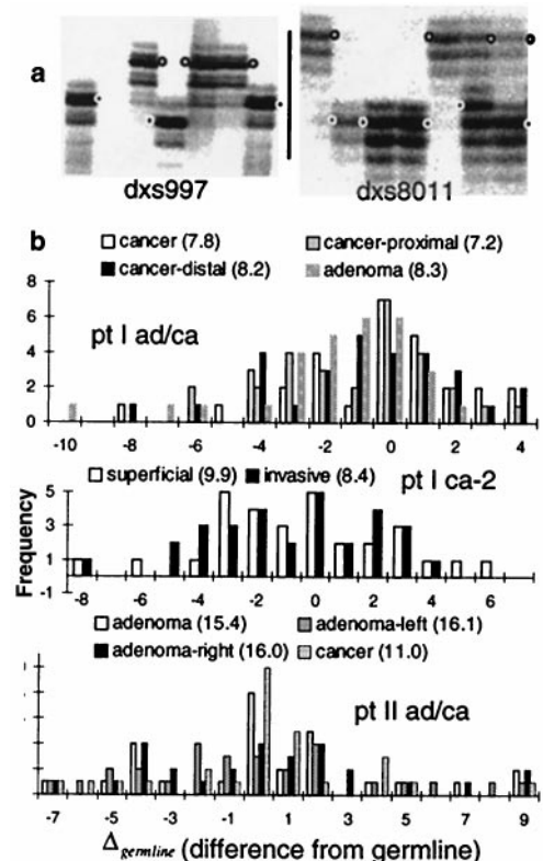
Fig. 3. (a) Autoradiographs of human tumor MS alleles. After dilution and PCR, the germline alleles (open circles) and tumor specific alleles (filled circles) become evident. Although the tumor alleles are polymorphic, they exhibit a modal size [−2 for DXS997 in the invasive cancer of Patient V (left) and −5 for DXS8011 in the right adenoma region of Patient II (right)]. (b) The differences from germline ( \Delta_{germline} ) of the 21–30 different MS loci from Patients I or II. Broader distributions, summarized by their variances ( S^2_{loci} in parentheses), indicate greater numbers of divisions since the loss of MMR (see Fig. 1 and compare with Fig. 2). Different regions from the same tumor have similar distributions and S^2_{loci} values.
