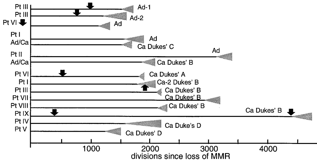
Fig. 4. Colorectal tumor histories inferred from their MS mutations. Each tumor history is unique, and most divisions occur before terminal clonal expansion (gray triangles). The average age is 2,300 divisions since loss of MMR. A trend toward increasing age with histologic progression is not apparent as the cancers and adenomas have similar ages. Negative clinical examinations (arrows, assuming one division per day) preceded six tumors, and for five tumors provided independent verification because they occurred before the postulated initiation of terminal clonal expansion. The negative examination in Patient I after the estimated initiation of the expansion of his Cancer-2 may indicate that it either was missed or was still too small to be detected. The data are consistent with genetic progression in the absence of visible progression, suggesting progenitor clone sizes are often below the threshold of clinical detection after loss of MMR.
