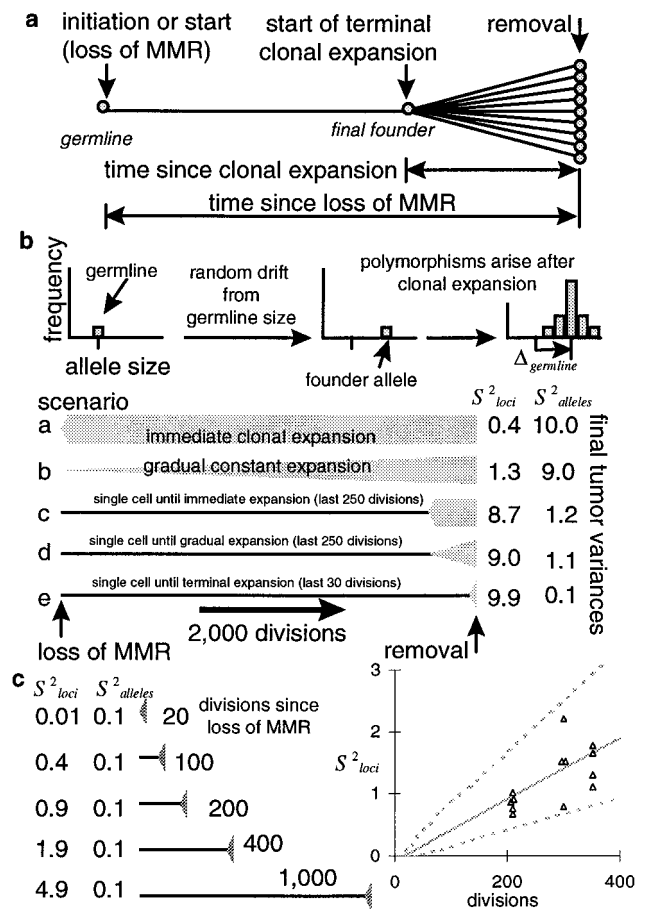
Fig. 1. (a) A tumor history is “read” from the mutations present in its cells. All of these cells are related to a single founder cell that represents the final bottleneck along a progression pathway. The history of this founder cell can be traced back along a single lineage because of the bottleneck nature of progression. We define the start of this pathway as the somatic loss of MMR. MS loci can record this history. Consider a single MS locus. After loss of MMR, the locus will randomly become larger or smaller, with the difference from its germline length a function of the number of divisions since loss of MMR. Upon terminal clonal expansion, the locus will become polymorphic. The time since terminal clonal expansion is reflected in the width or variance ( S_{alleles}^2 ) of the tumor allele frequency distribution. The MS allele in the founder cell can be inferred by the most common allele present in the tumor. The time since loss of MMR preceding the bottleneck is reflected in the difference ( \Delta_{germline} ) between the length of the germline allele and the founder allele. Although the stochastic nature of mutation makes a single MS locus relatively uninformative, the analysis repeated at 20–30 different loci is robust. (b) Simulations of MS mutation. Data represents the results of 1,000 trials with 20–30 MS loci, and a symmetric stepwise model with the chance of addition of one repeat of 0.0025, and loss of one repeat of 0.0025, with the total mutation rate of 0.005 per division. In each scenario, the final tumor size is 1.0 cm 3 or one billion cells. Different patterns of MS mutations, summarized by the variances, S_{alleles}^2 and S_{loci}^2 , are obtained with identical numbers of divisions (2,000) but different tumor histories. Therefore, a history of a human tumor can be inferred by sampling its MS alleles and estimating S_{alleles}^2 and S_{loci}^2 . (c) Example of simulations with identical clonal expansion histories (20 terminal exponential divisions) but different times since loss of MMR. The average value of S_{loci}^2 increases with the numbers of divisions since loss of MMR whereas S_{alleles}^2 is constant. The graph illustrates the mean and 95% confidence intervals (dotted lines) of the simulations. The triangles in the graph represent values obtained from 210- to 352-day-old tissue culture experiments that mirror these simulations (see Fig. 2).
